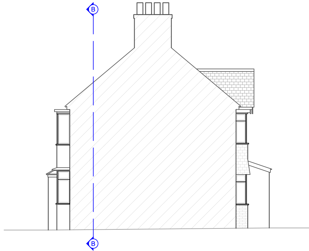
Side (East) Elevation
