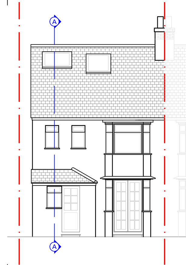
Rear Elevation
