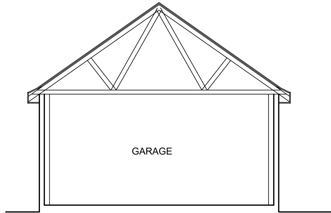
SECTION AS EXISTING
