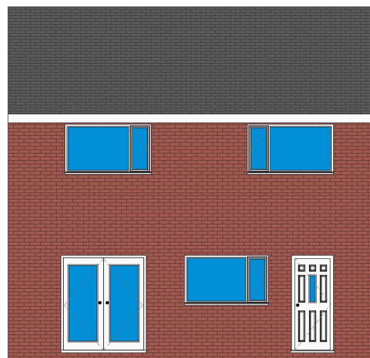
4 Existing Rear Elevation 1 : 50
