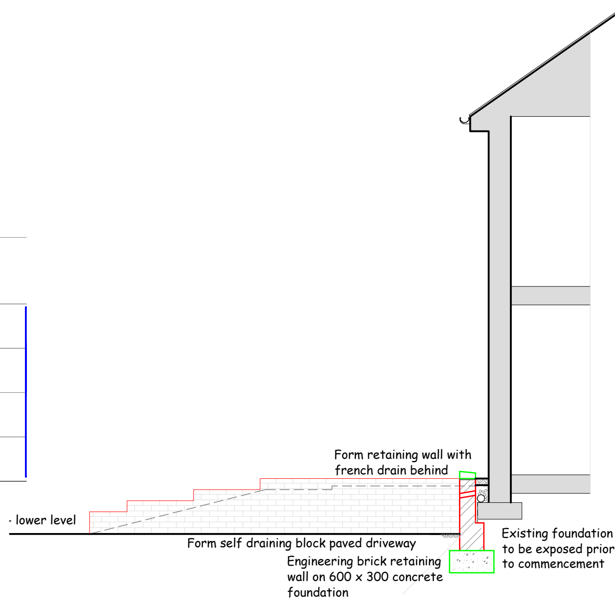
Section 1:50
