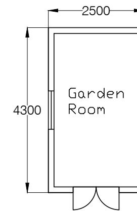
Floor Plan (Proposed)
