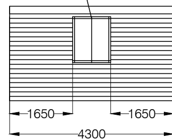
Rear Elevation (Proposed)
