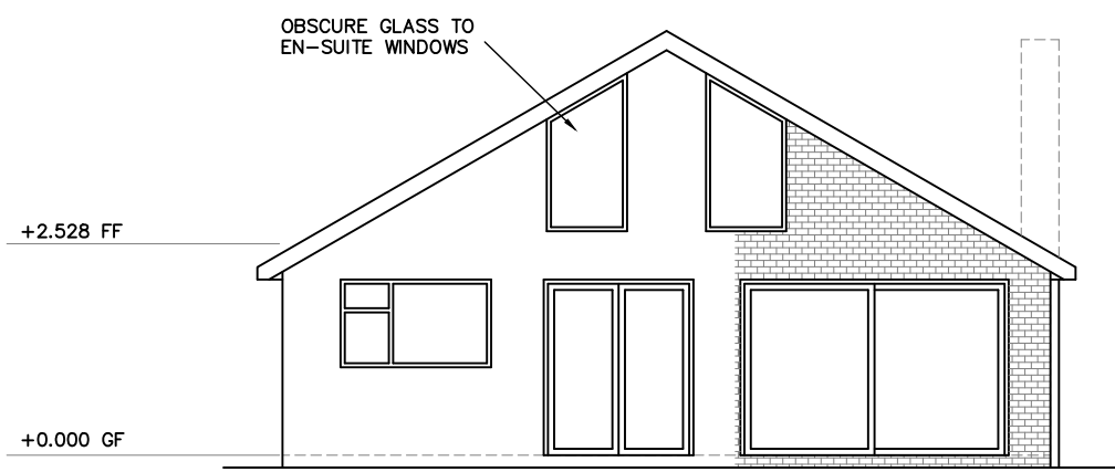
REAR ELEVATION
