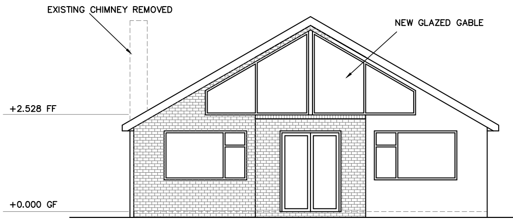
FRONT ELEVATION
