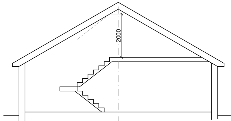
TYPICAL SECTION THROUGH STAIRCASE
