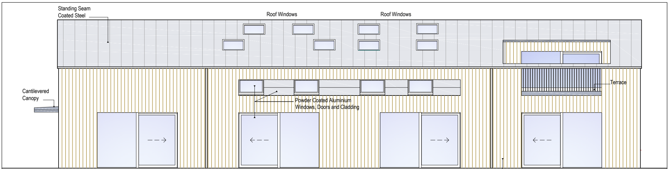
APPROVED SOUTH ELEVATION
