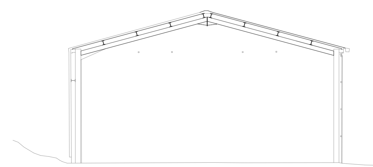
Cross Section Existing 1 : 100
