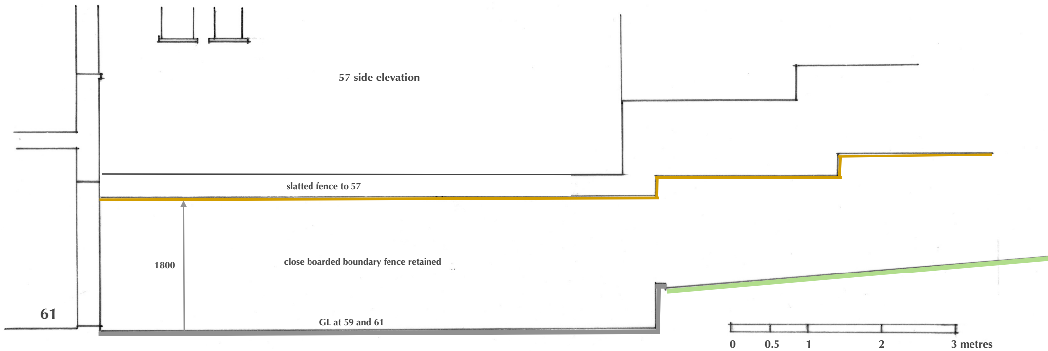
South Elevation at boundary with 61 showing boundary fence
