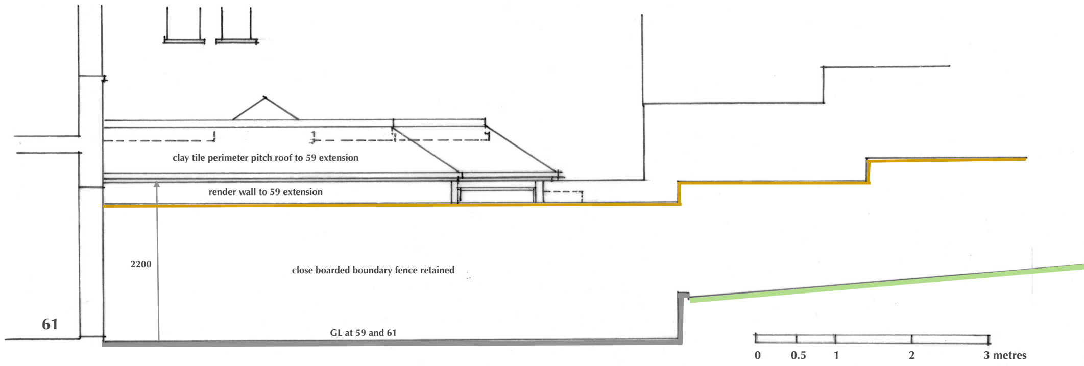
South Elevation at boundary with 61
