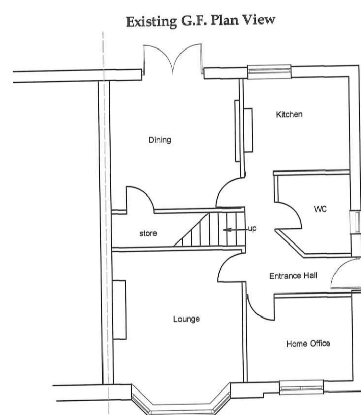
Existing G.F. Plan View
