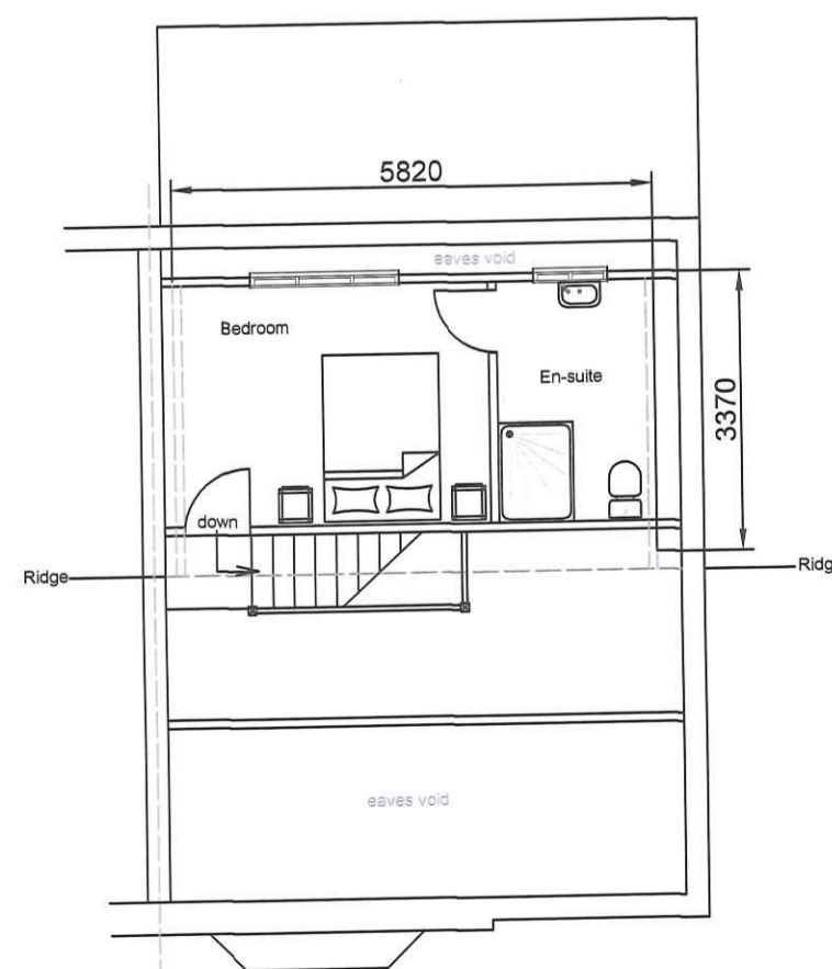
Proposed 2nd Floor Plan View
