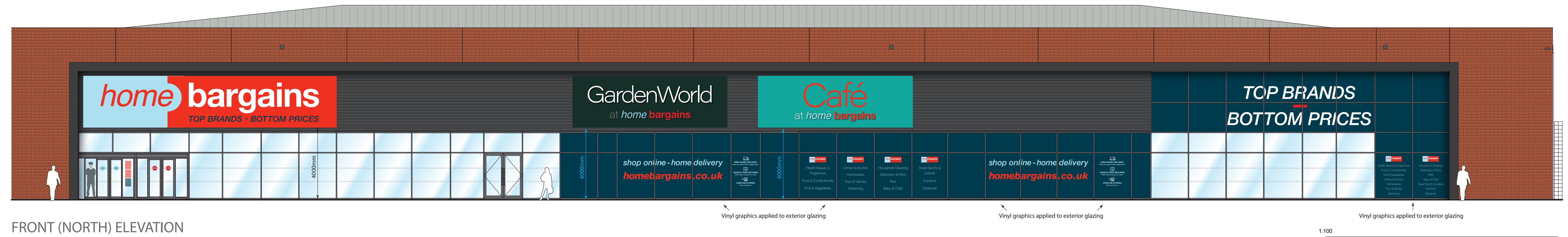
Sign A Size: 13100mm x 2660mm Sign weight: 280kg
