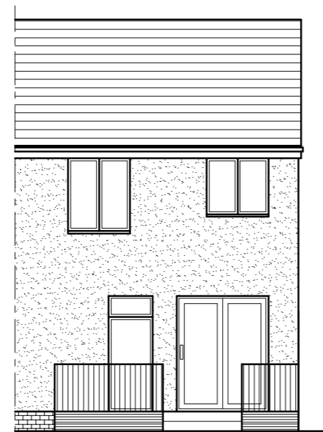
Rear 1:100
