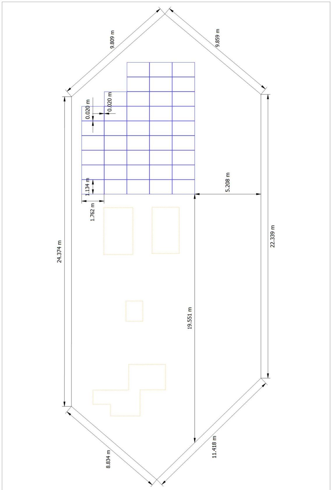
Figure: Arbitrary Building 06 - Mounting Surface Southwest
