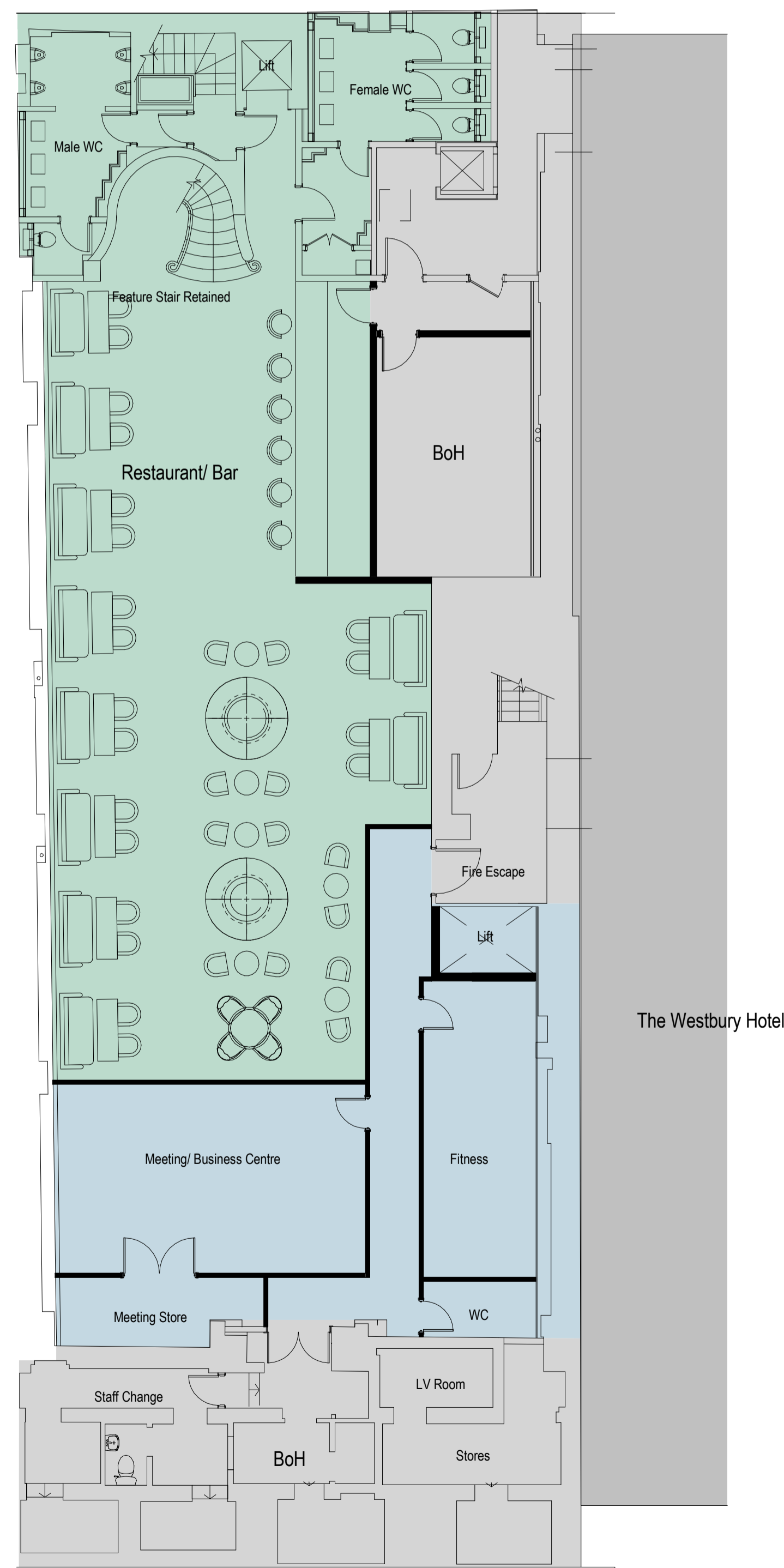
2 B1-Plan Washington. General Arrangement 1 : 100
