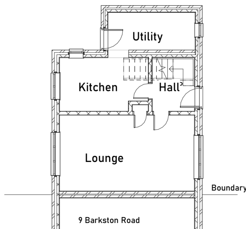
1 Level 2 Ground Floor 1 : 100
