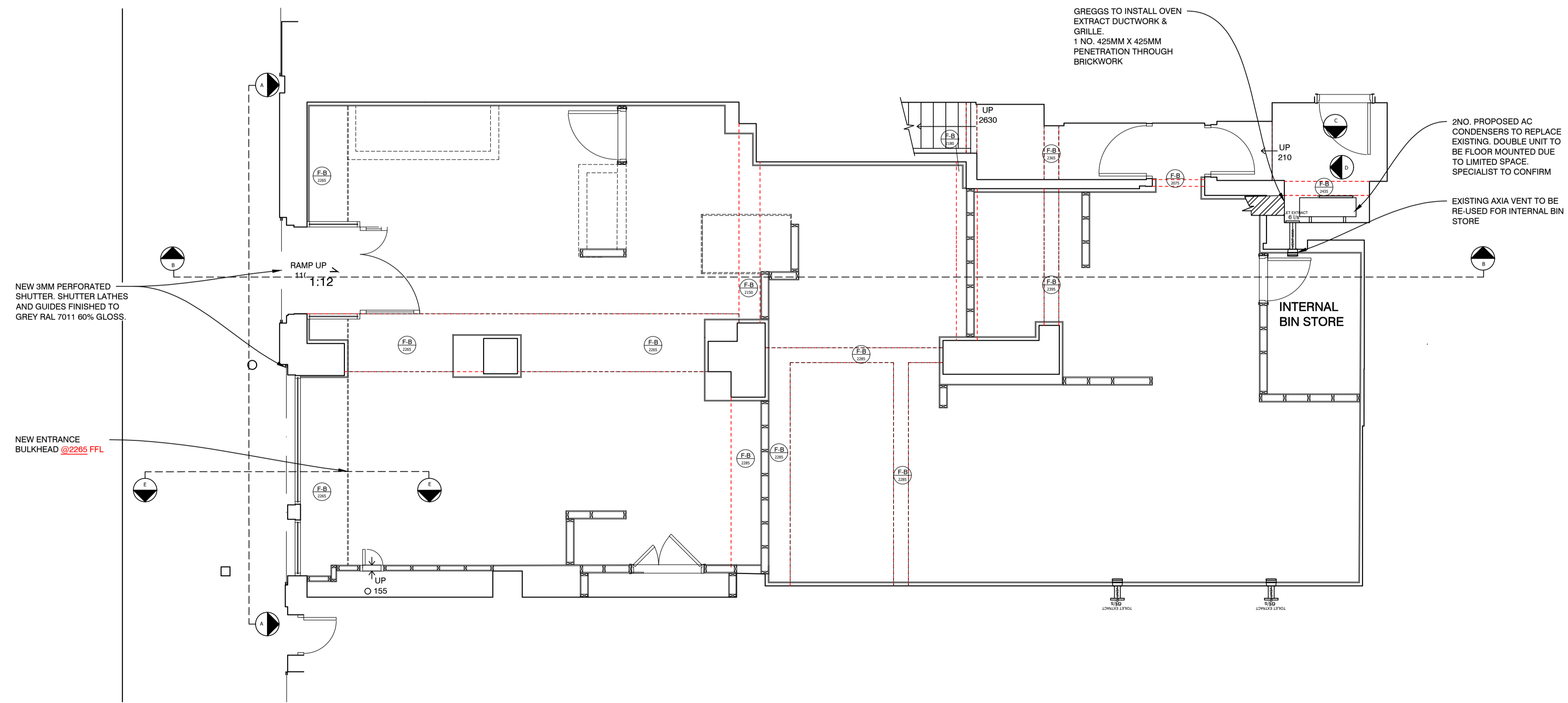
GROUND FLOOR - PROPOSED GA PLAN (1:50)
