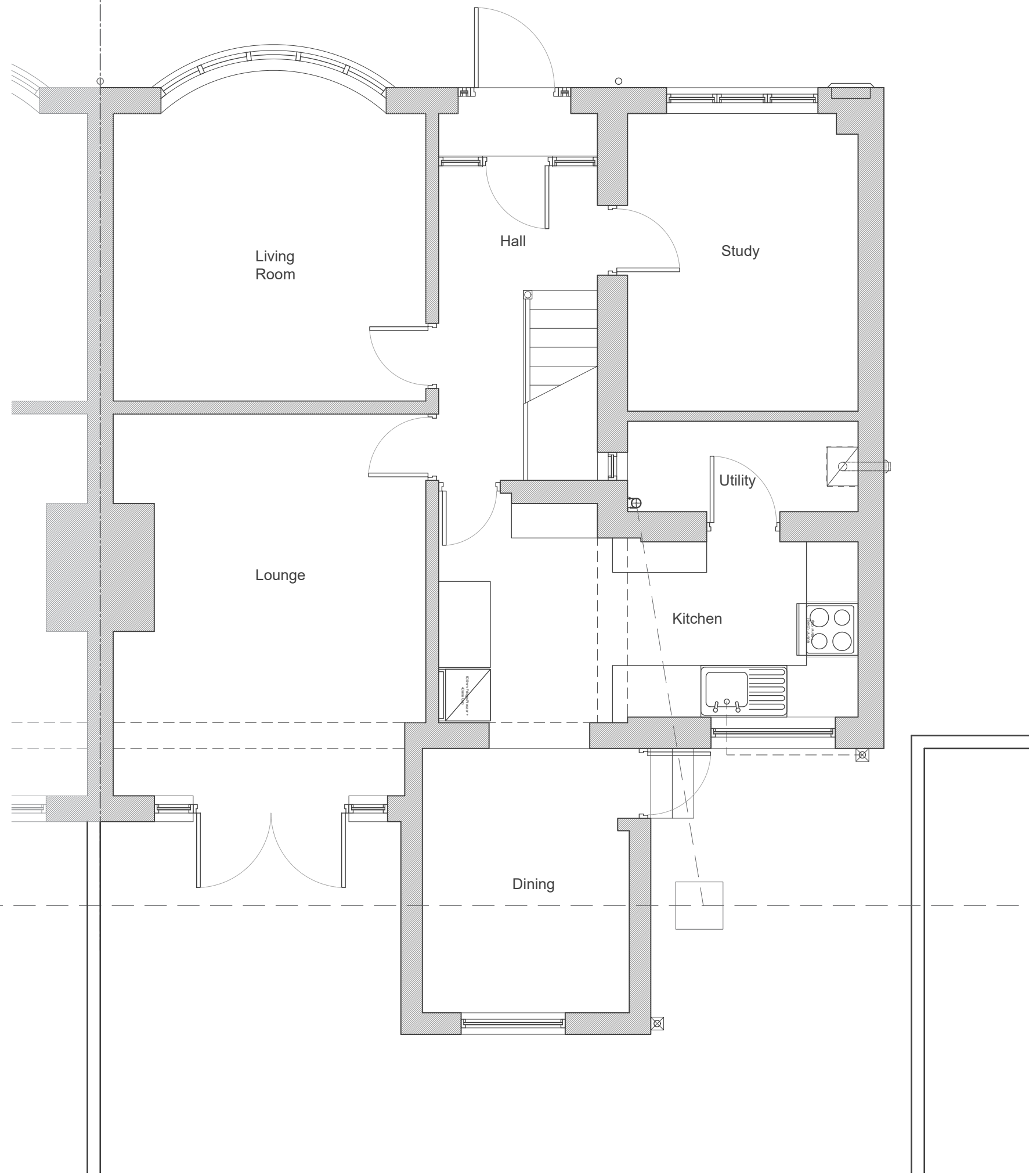
Ground Floor 1:50
