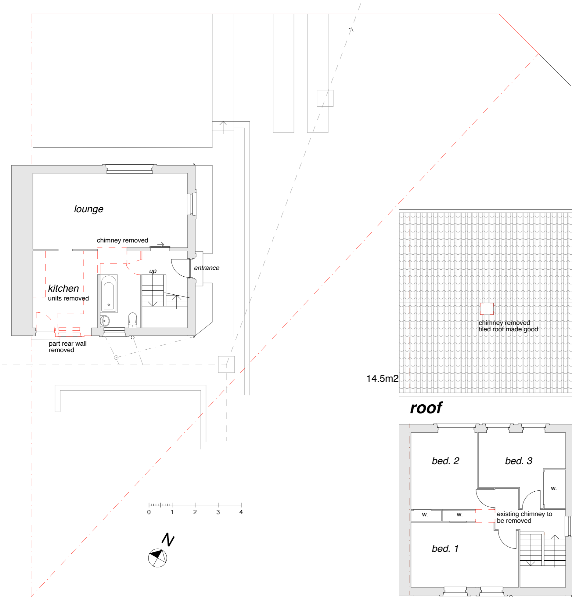
ground floor and site plan
