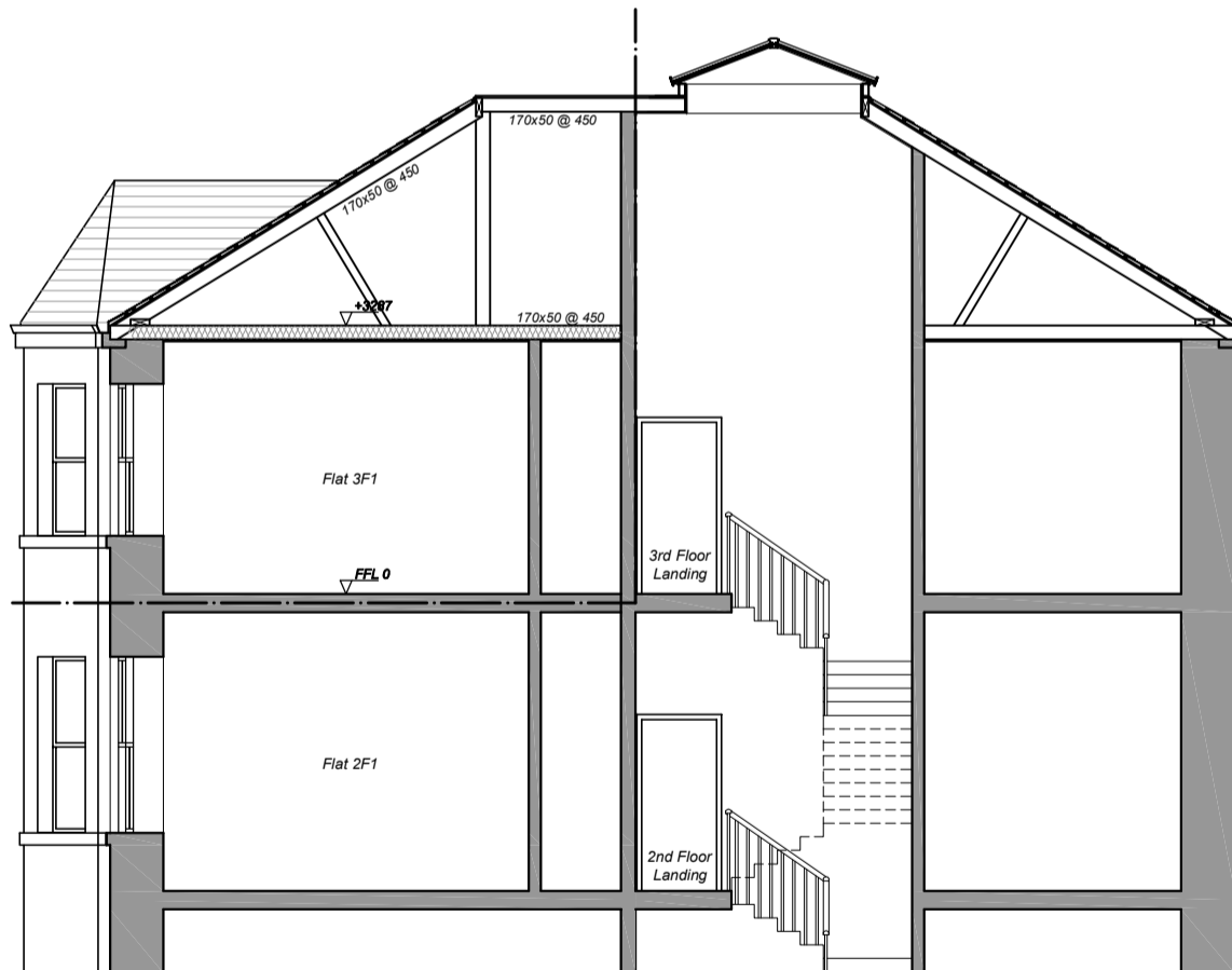
Section B-B as Existing
