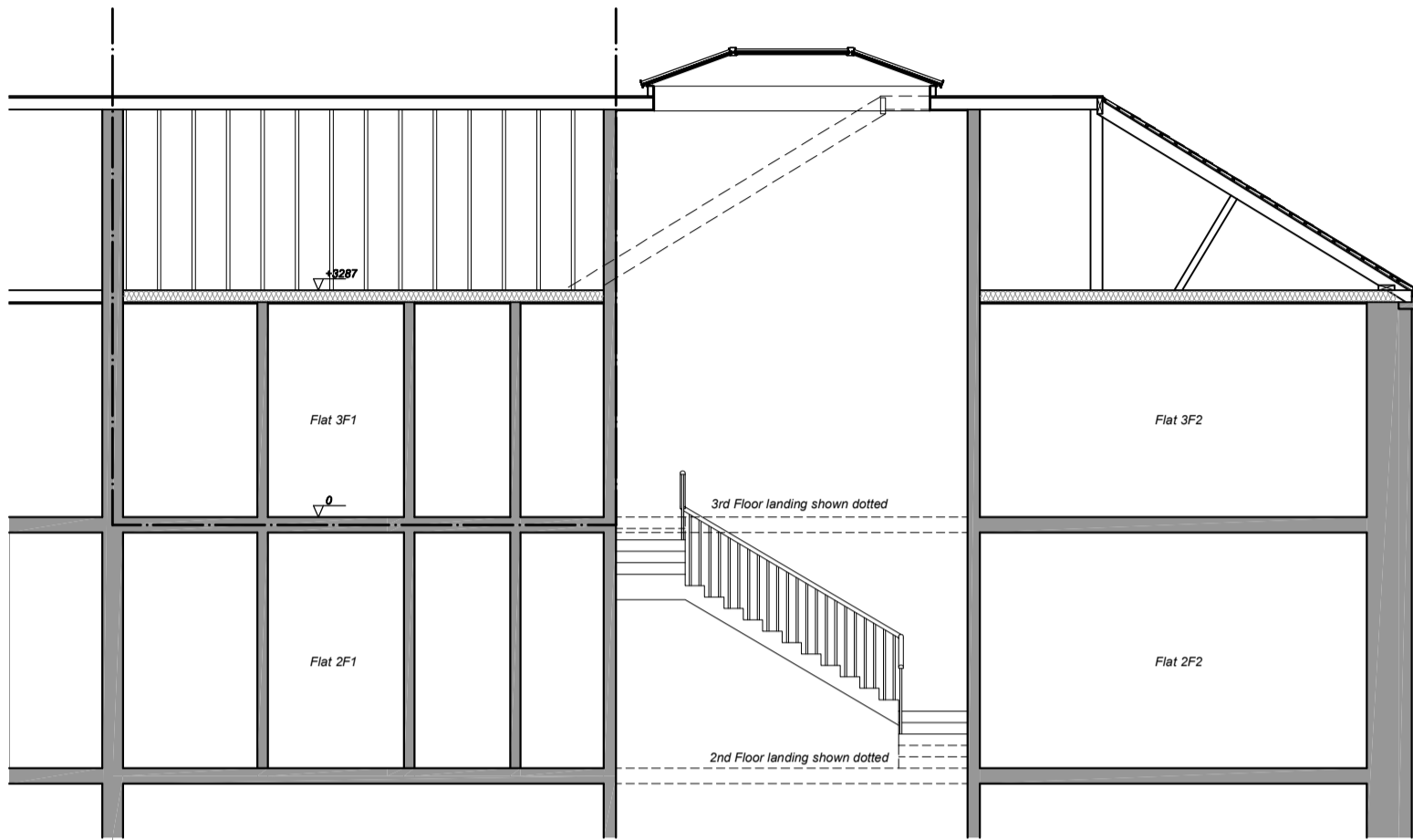
Section A-A as Existing
