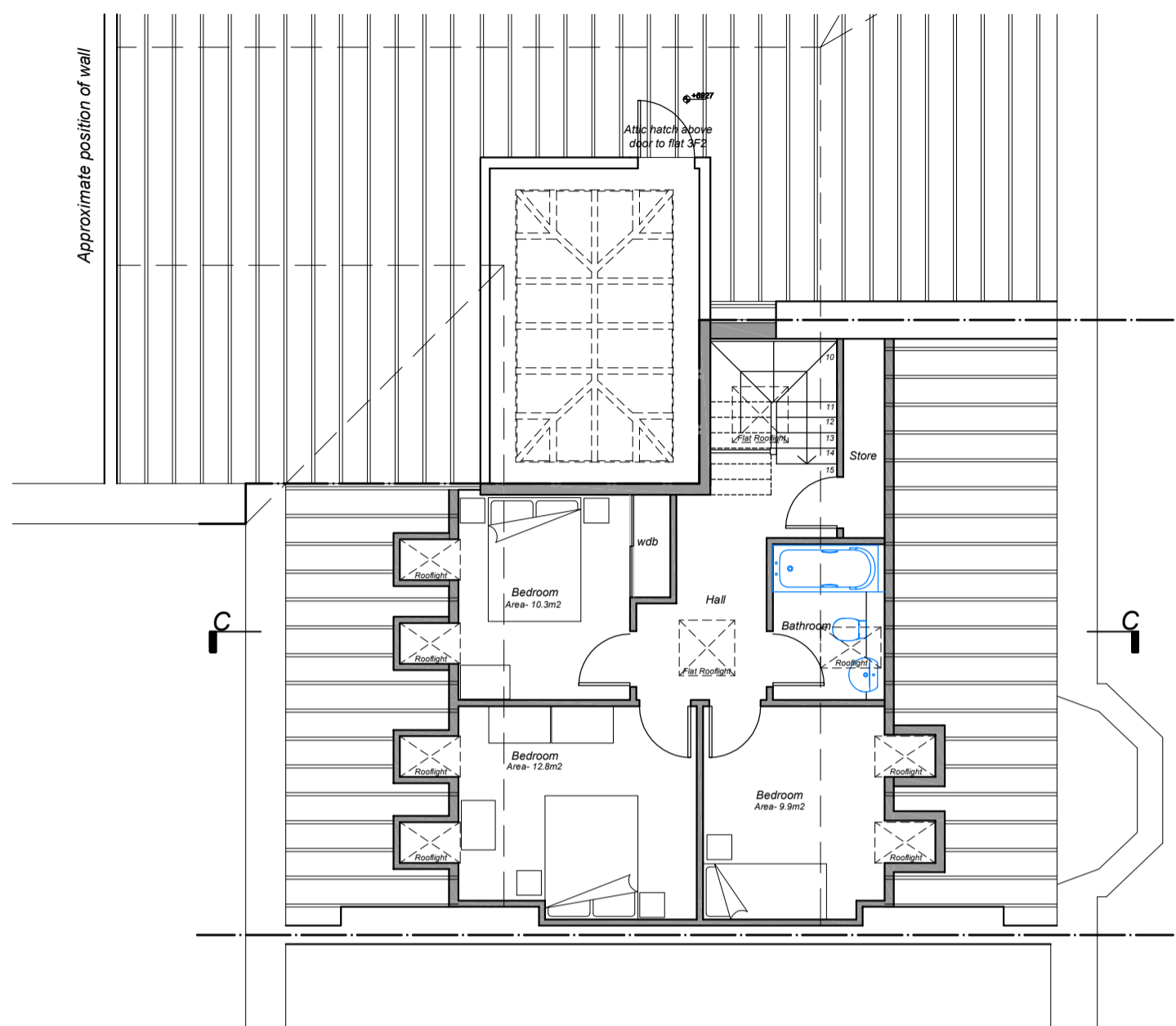
Flat 3F1 Attic Plan as Proposed
