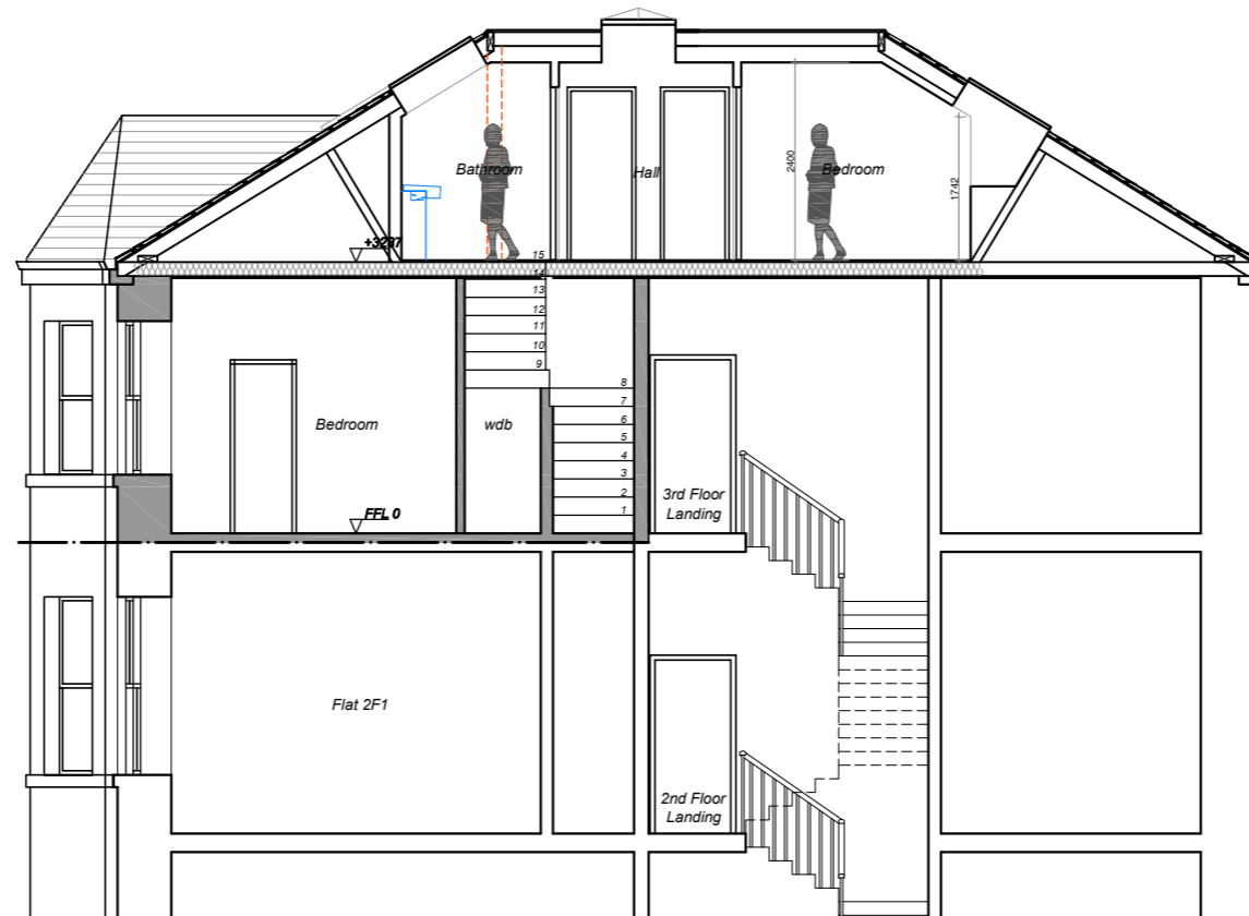
Section C-C as Proposed
