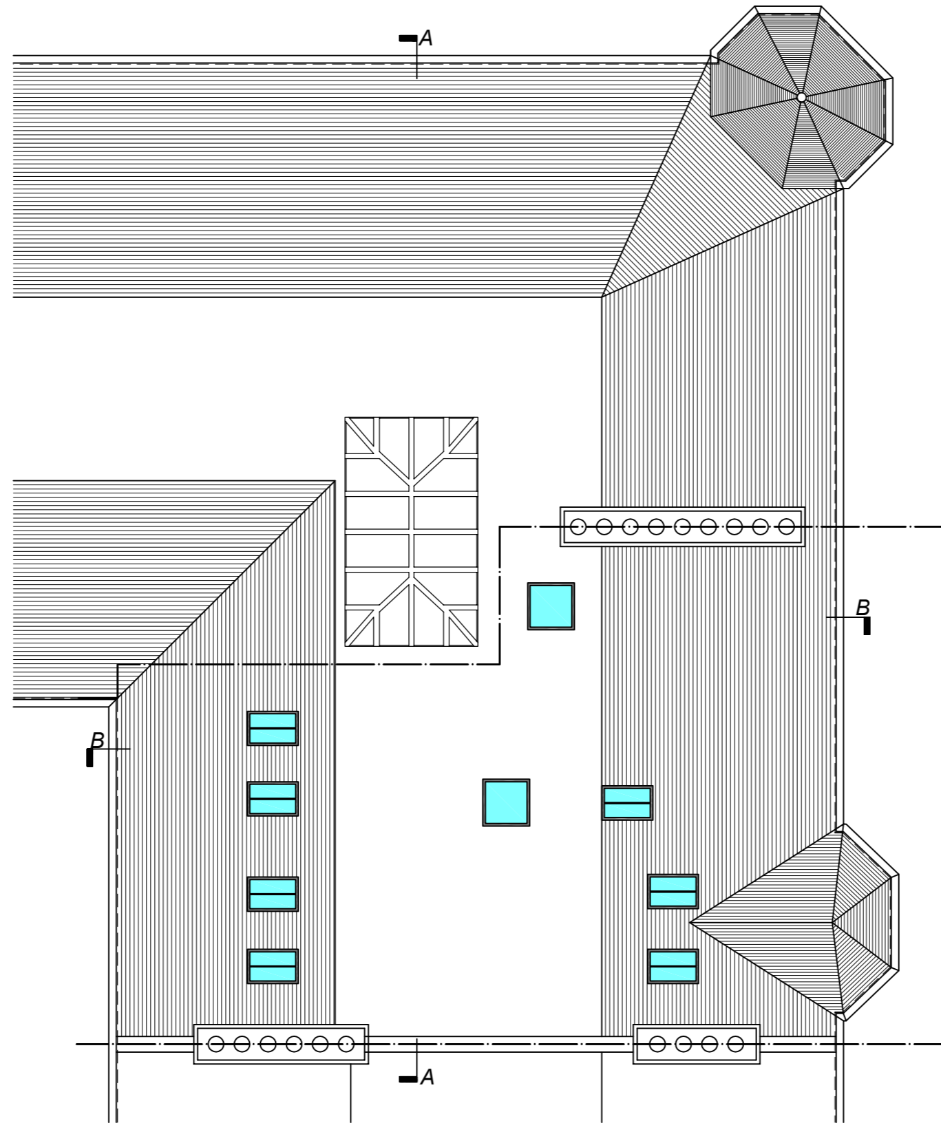
Roof Plan as Proposed
