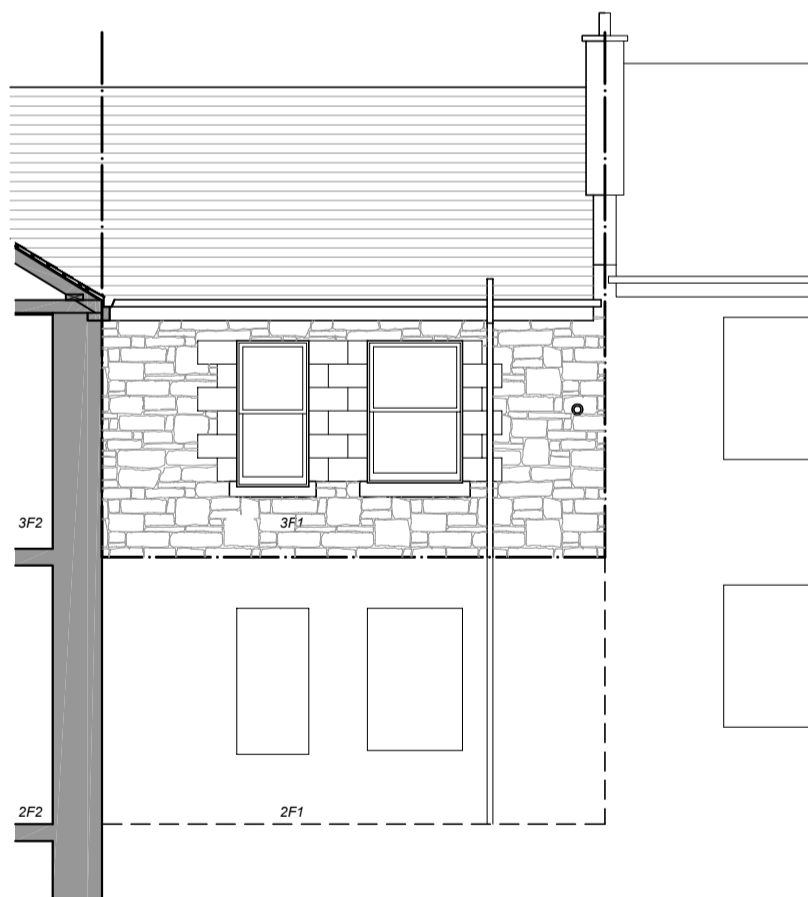
West Elevation (part) as Existing
