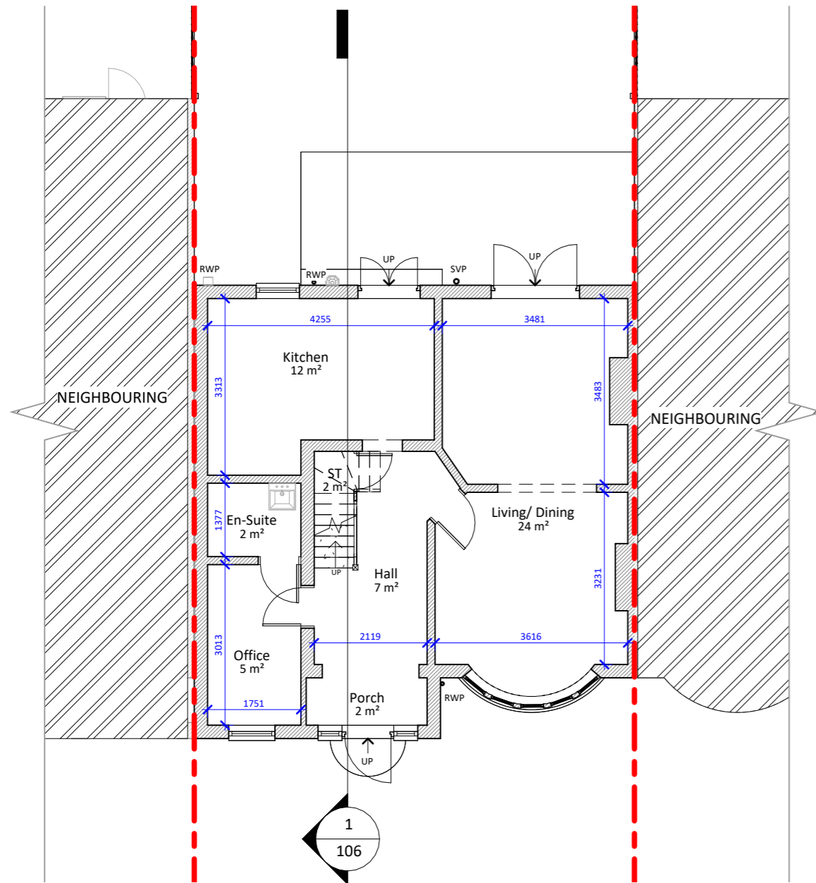
1 Existing Ground Floor 1 : 100
