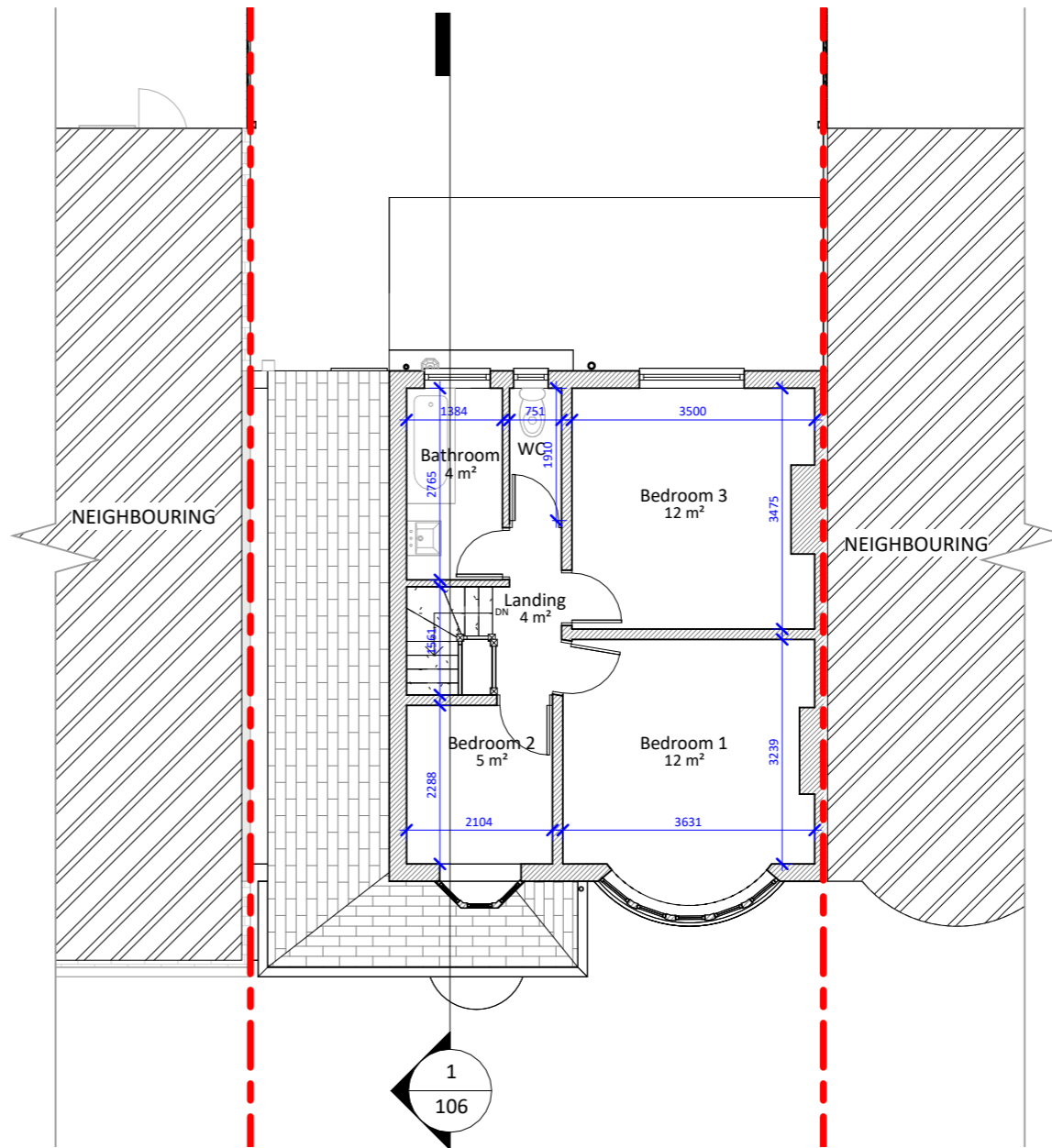
2 Existing First Floor 1 : 100
