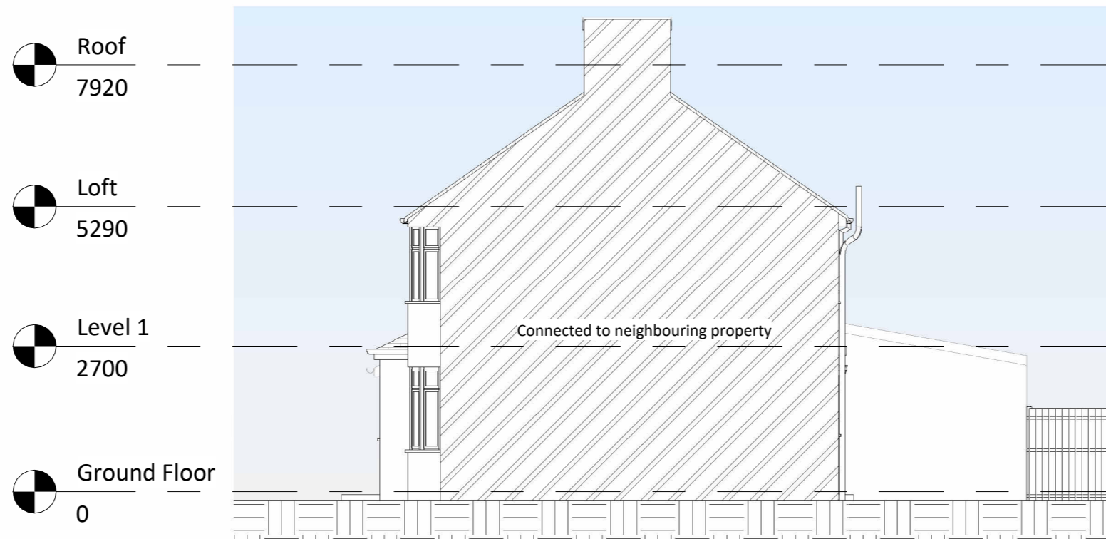
1 Existing Right Elevation 1 : 100
