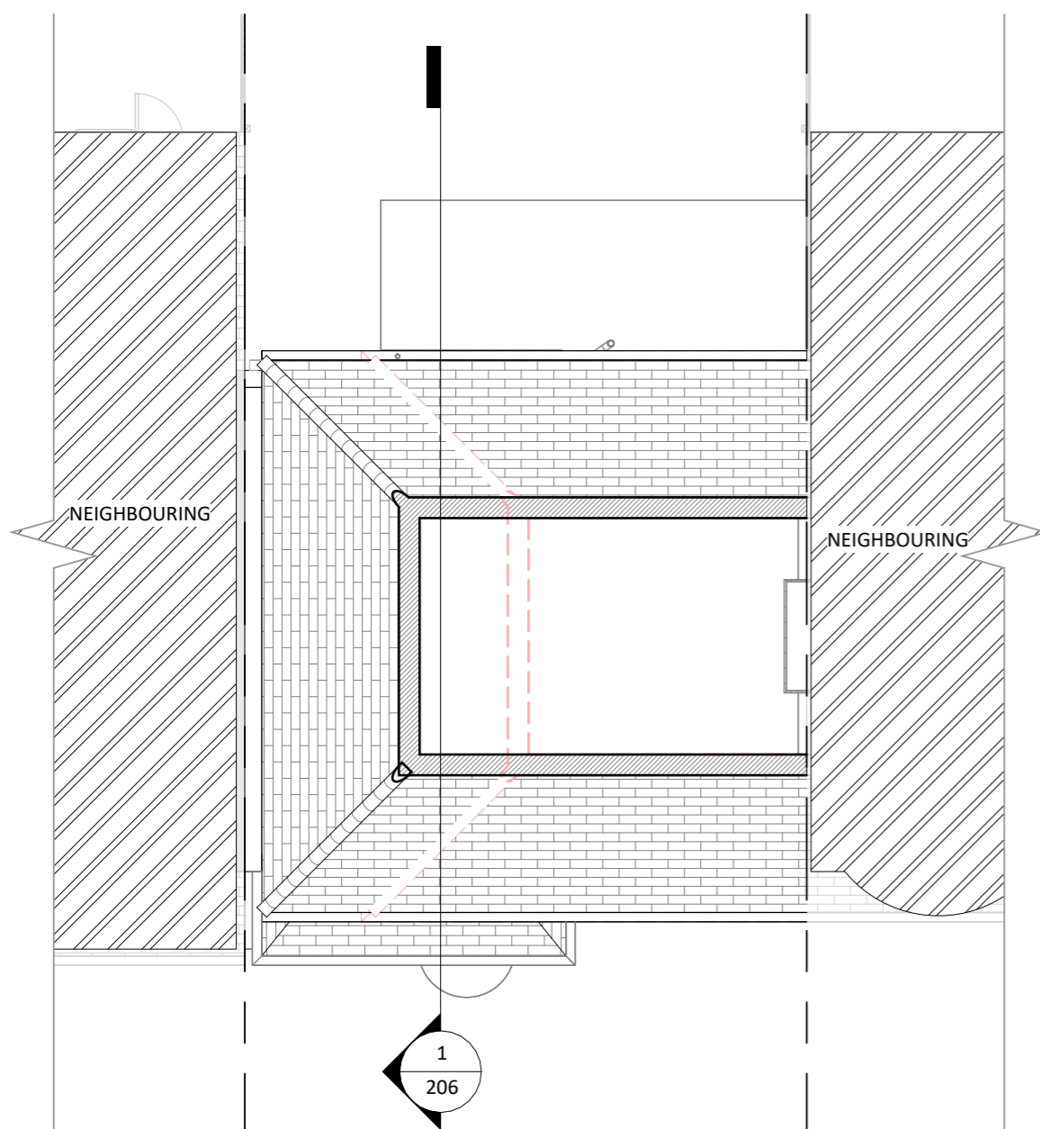
1 Loft (Proposed) 1 : 100
