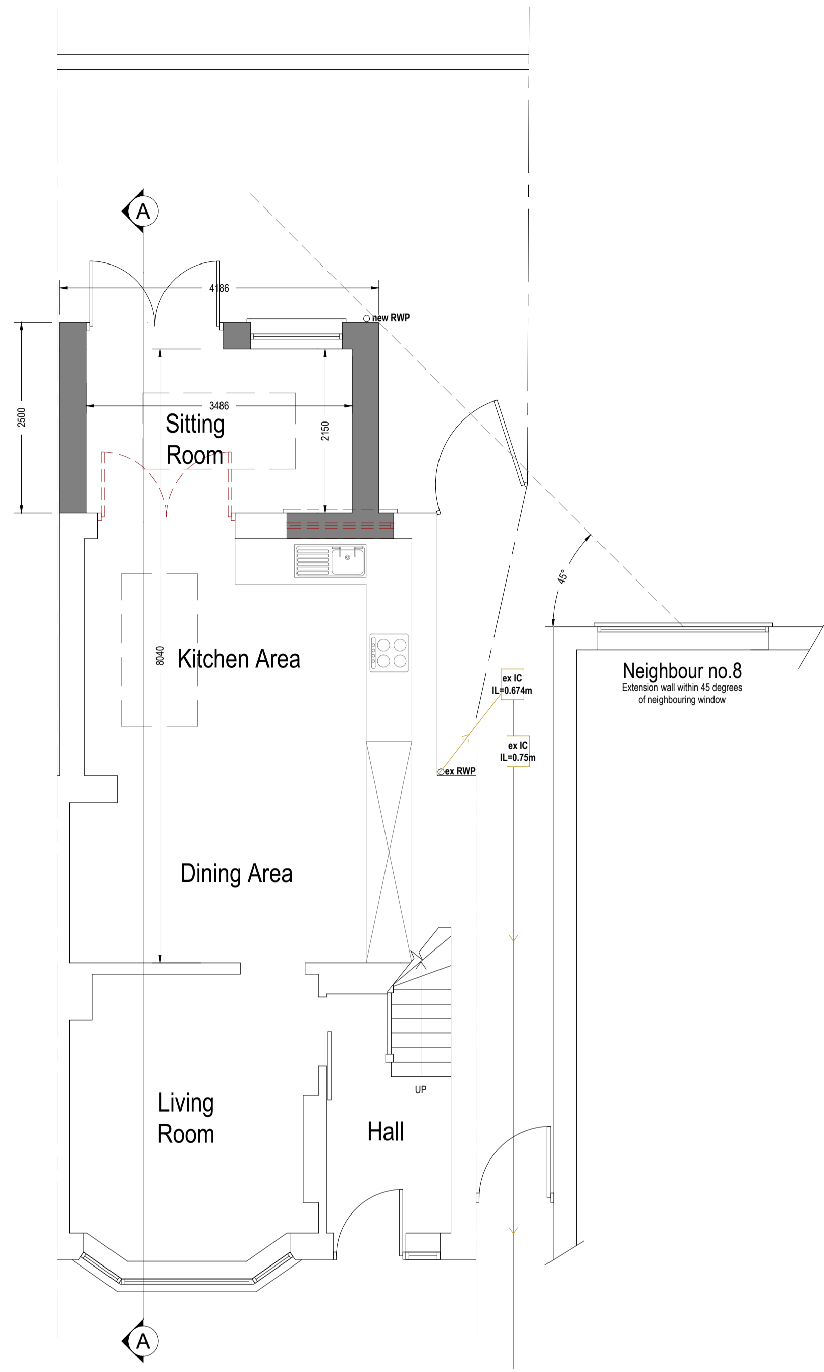
Ground Floor Plan Area ca. 51.39 m 2 Additional Area: 8.64 m 2
