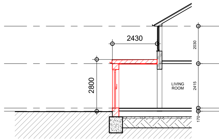
SECTION - EXISTING 5 1:100
