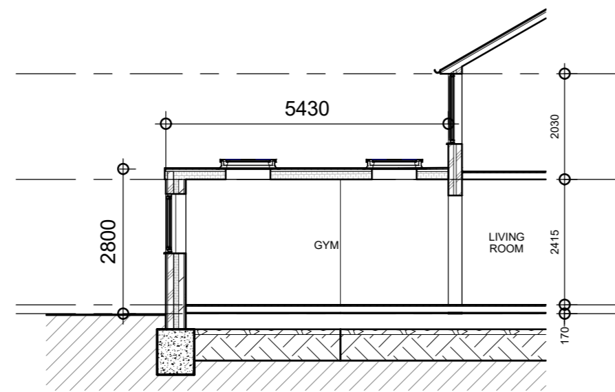
SECTION - PROPOSED 4 1:100
