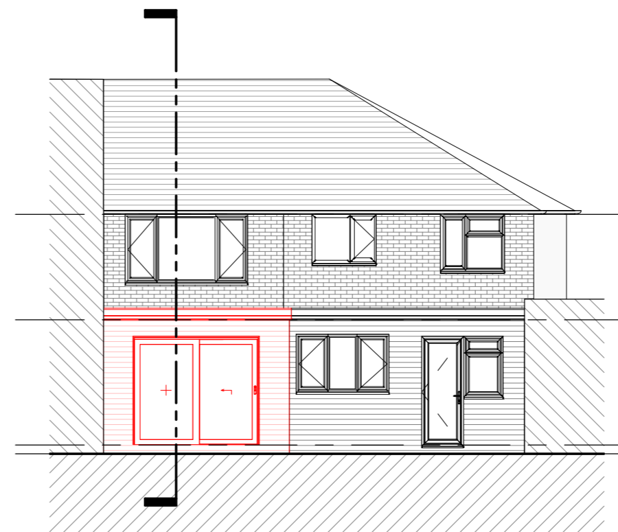
REAR ELEVATION - EXISTING 2 1:100
