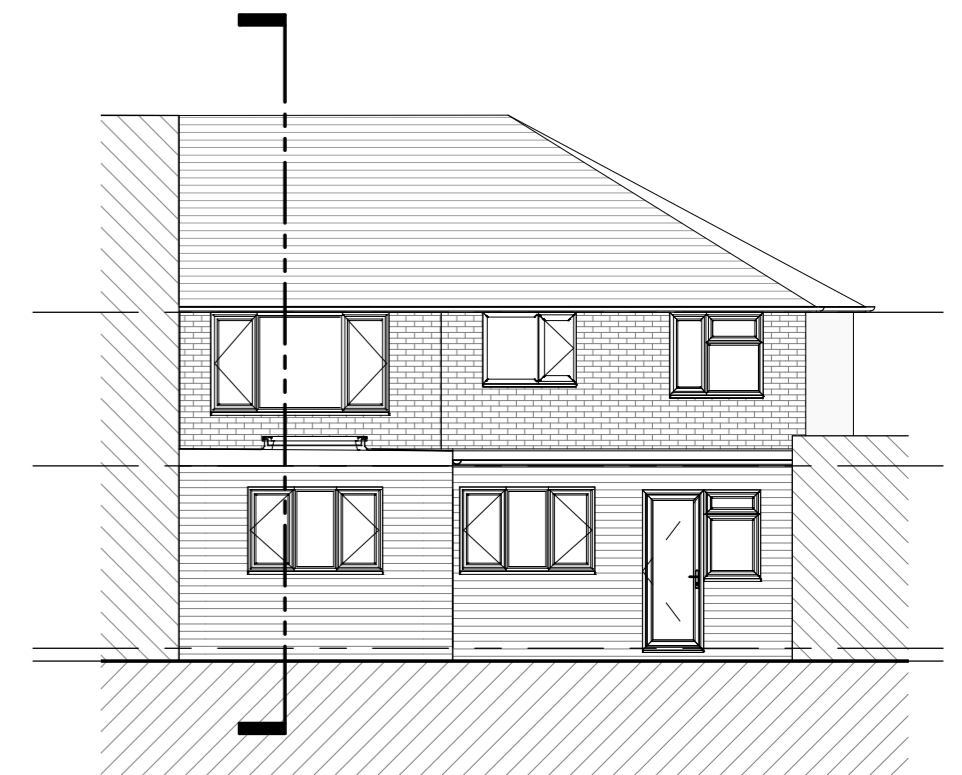
REAR ELEVATION PROPOSED 1 1:100
