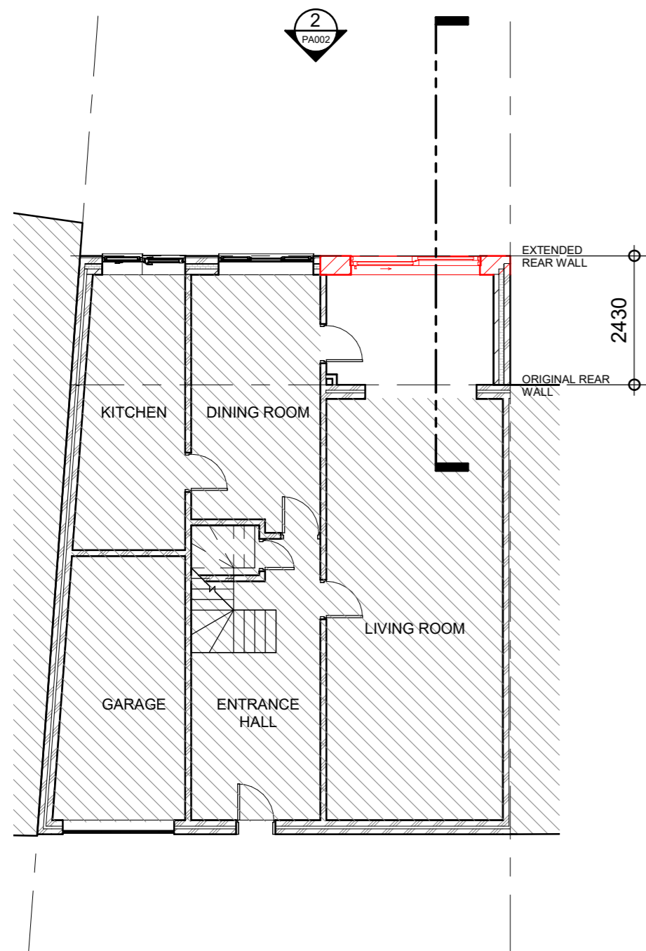
GROUND FLOOR EXISTING 7 1:100
