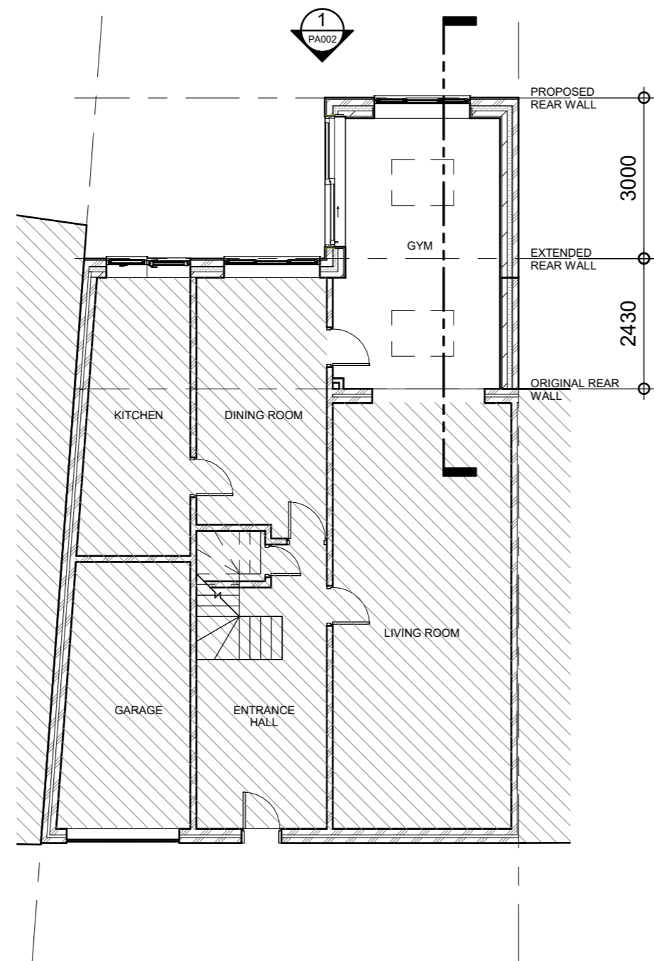
GROUND FLOOR - PROPOSED 6 1:100
