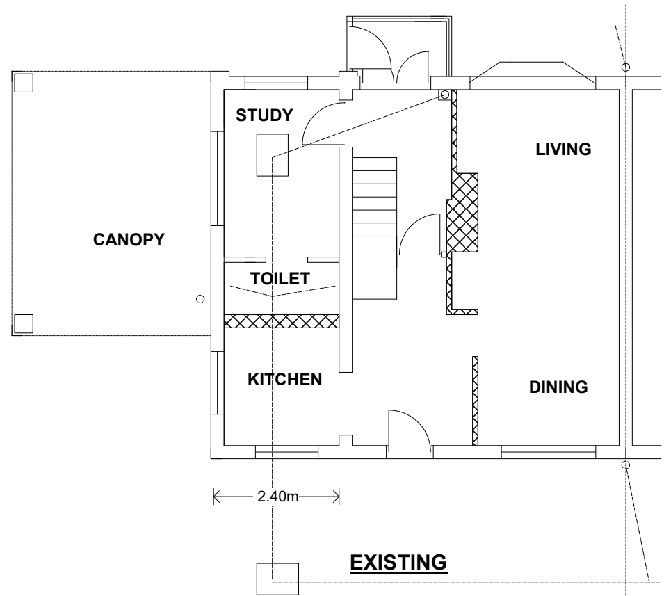
1:100 GND FLOOR LAYOUT
