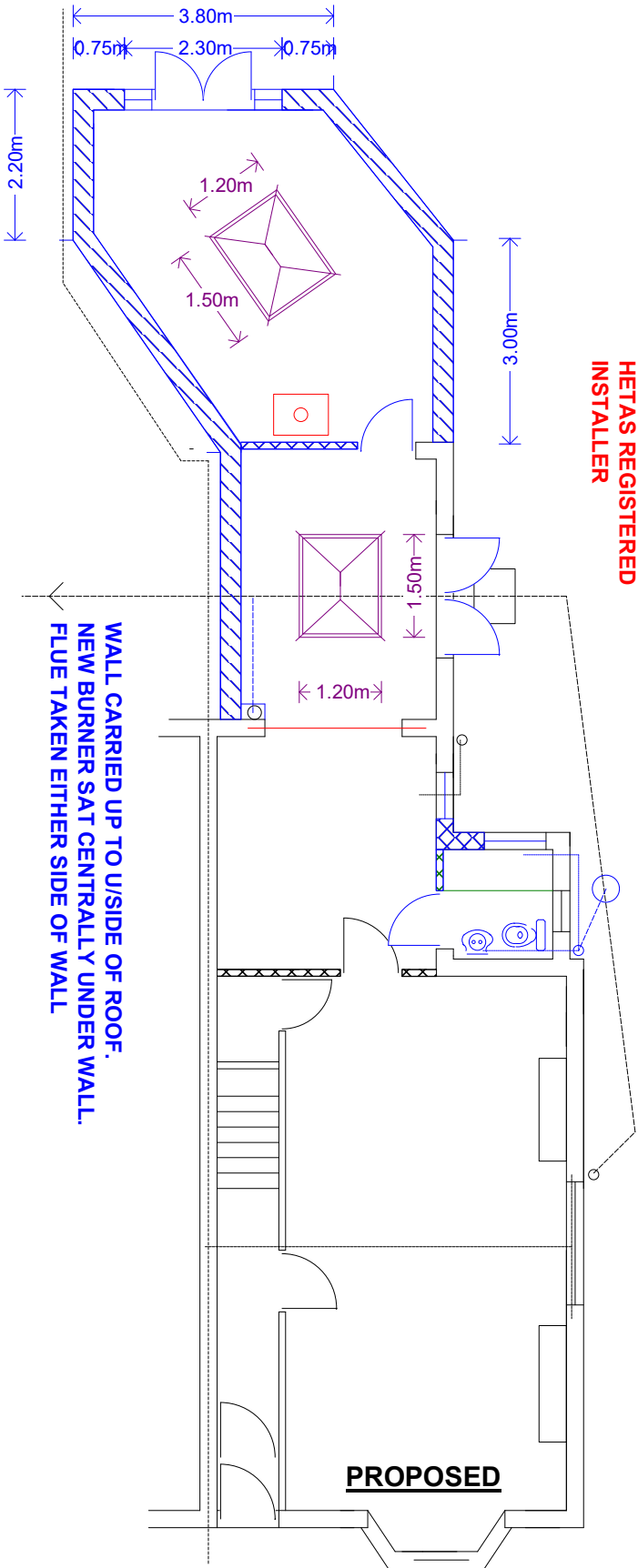
1:100 GND LAYOUT
