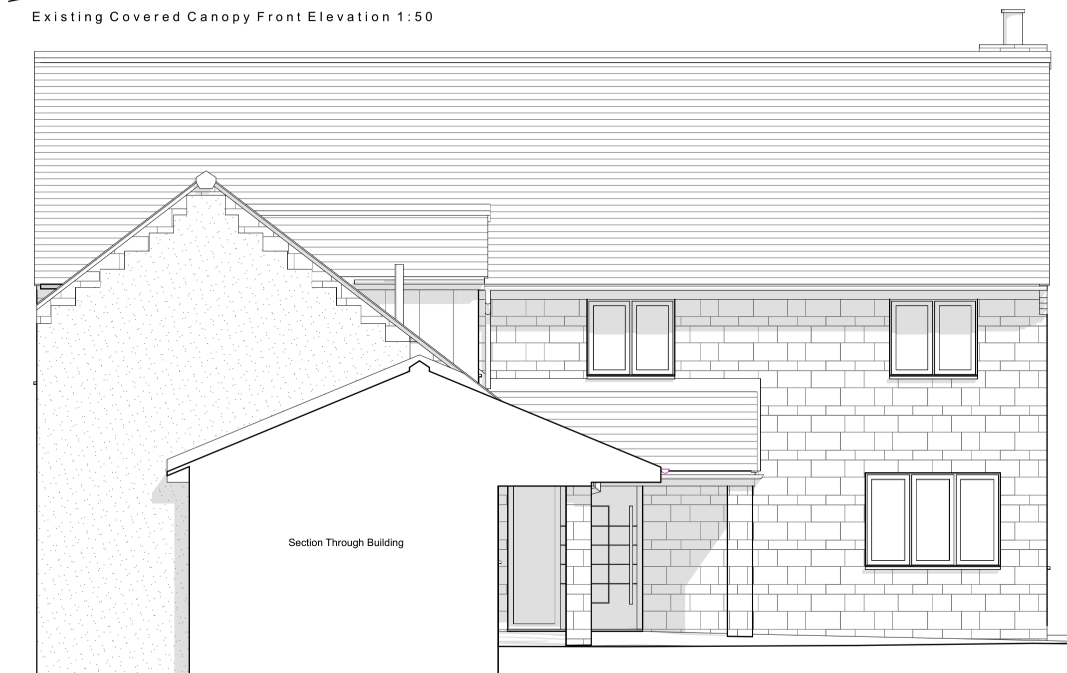
Existing Covered Canopy Side Elevation 1:50
