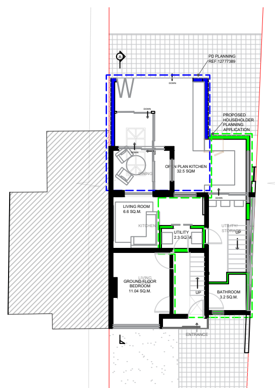
KEY PLAN | 1:200
