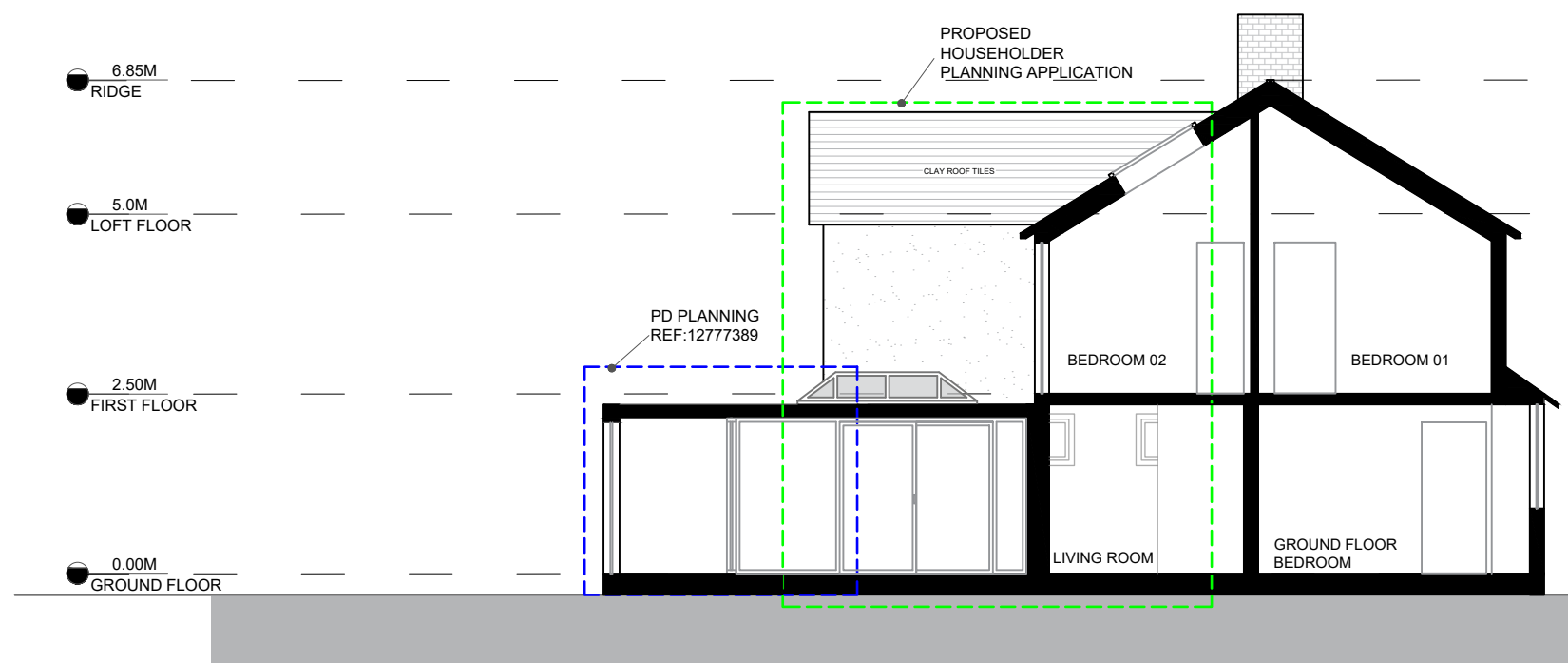
SECTION AA | 1:100
