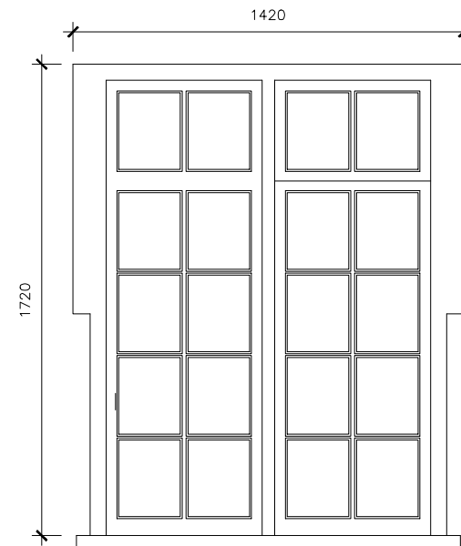
Window Assembly GW1
