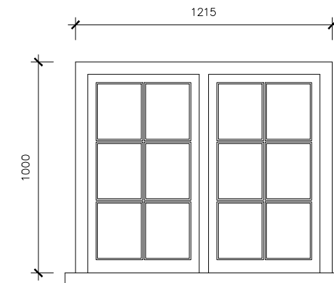
Window Assembly GW2
