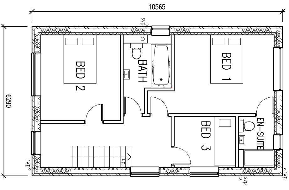
FIRST FLOOR PLAN (55m 2 )
