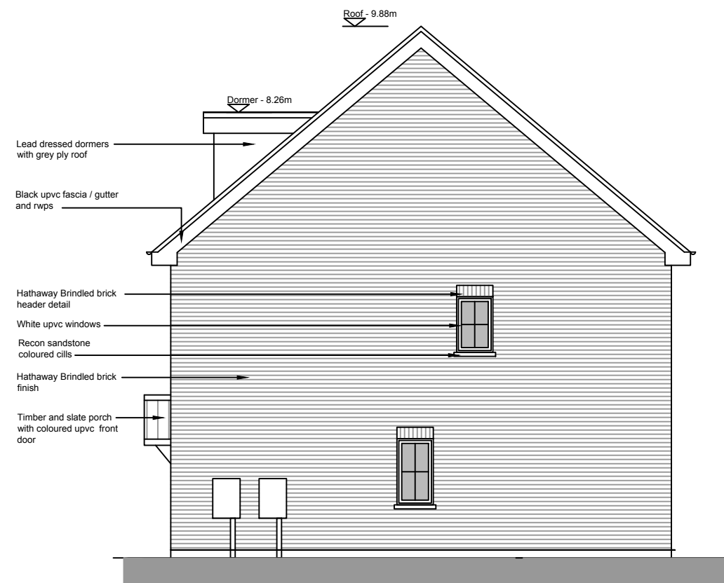
PROPOSED SIDE ELEVATION 2
