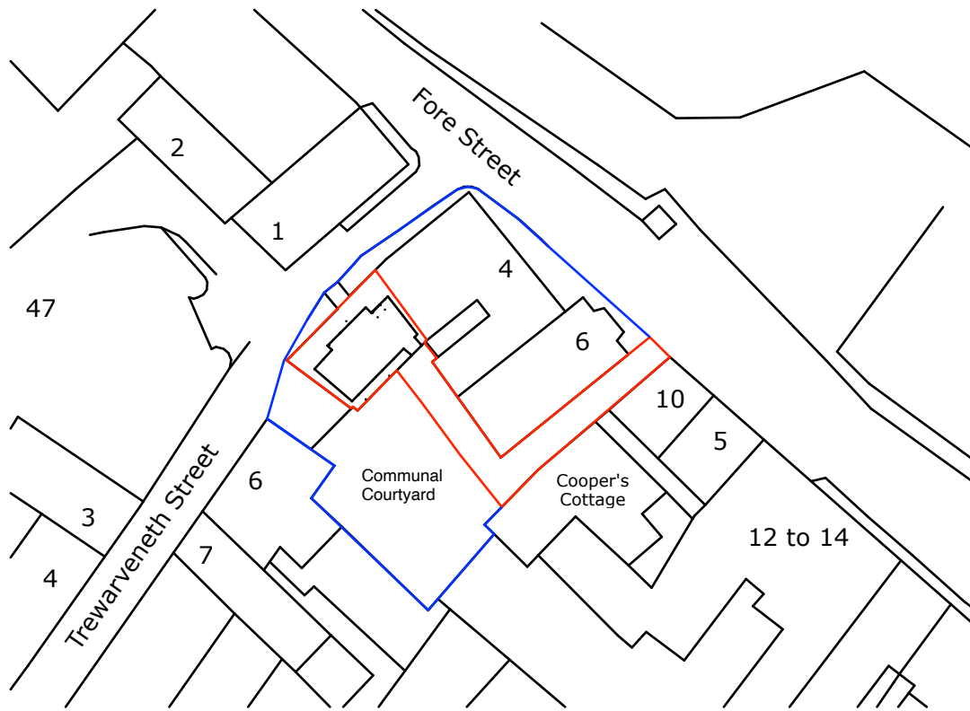
Site Layout (Block Plan) 1:500
