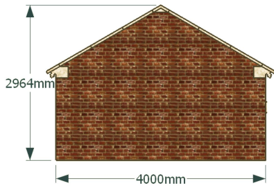
Rear Elevation
