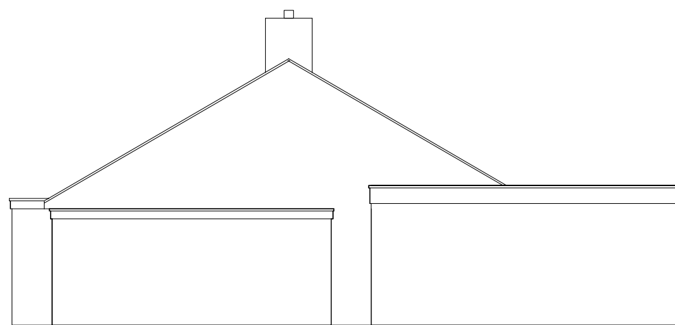
EXISTING SIDE ELEVATION (RIGHT)
