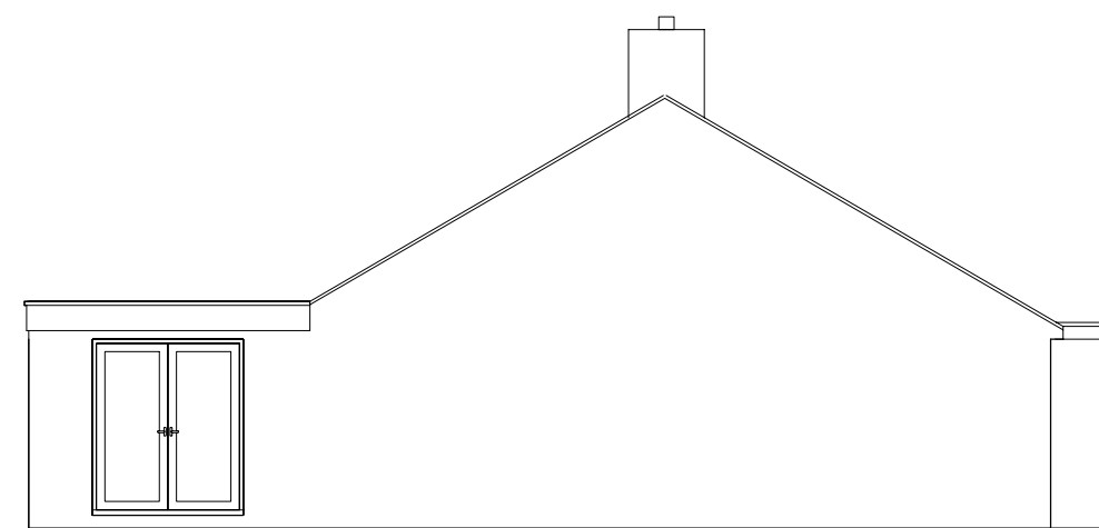
EXISTING SIDE ELEVATION (LEFT)
