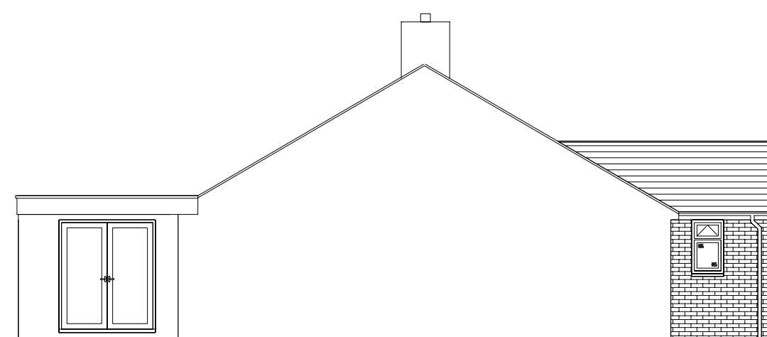
PROPOSED SIDE ELEVATION (LEFT)
