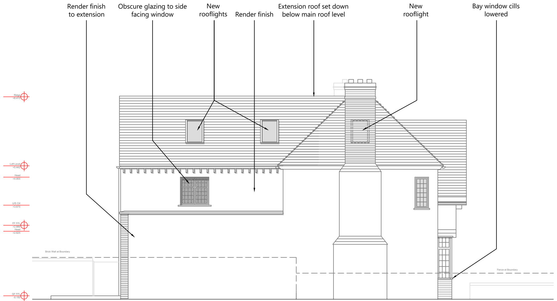
South-West Elevation Scale 1/100
