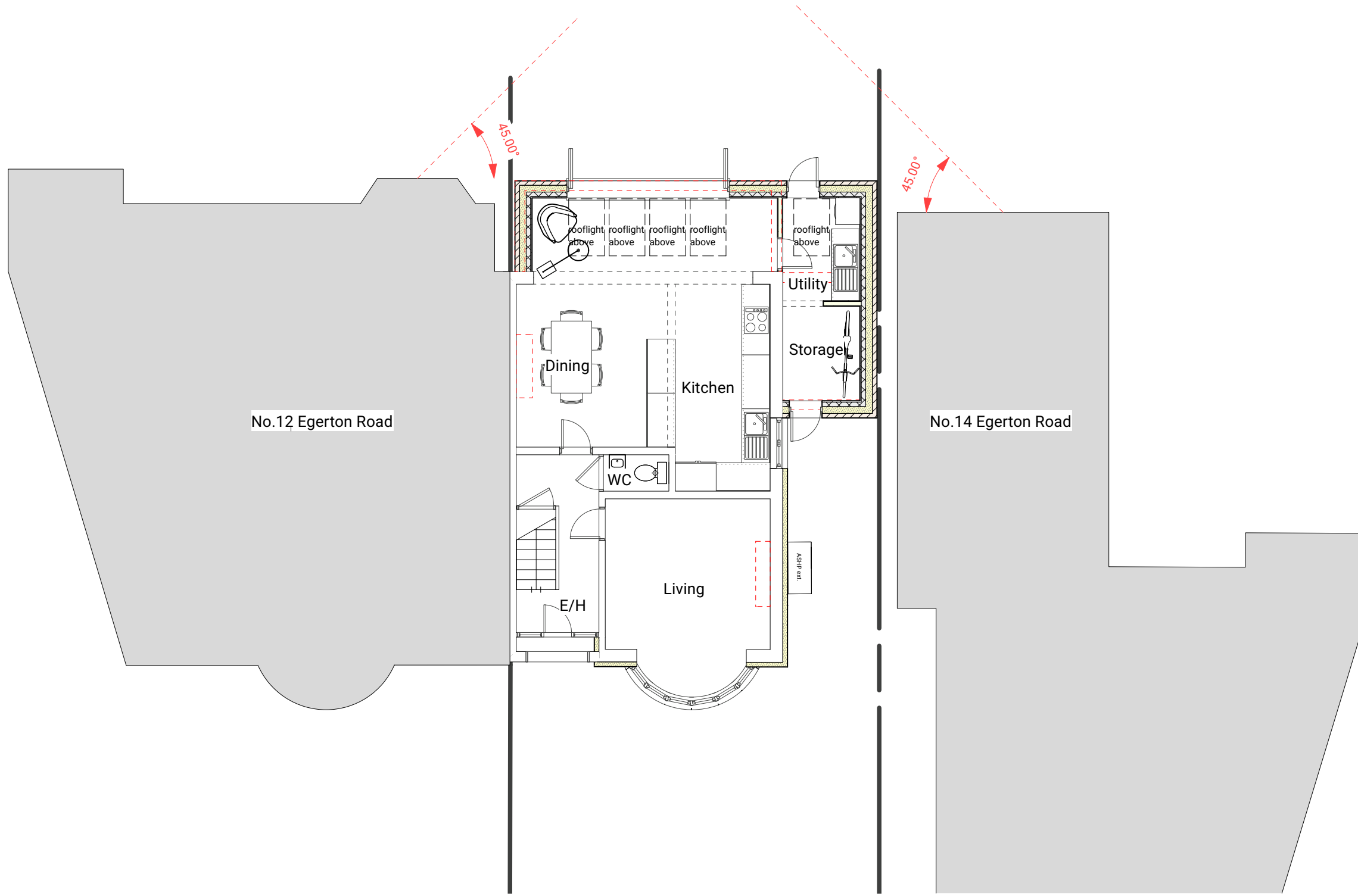
1 45 degree rule - Plan view Scale: 1:100
