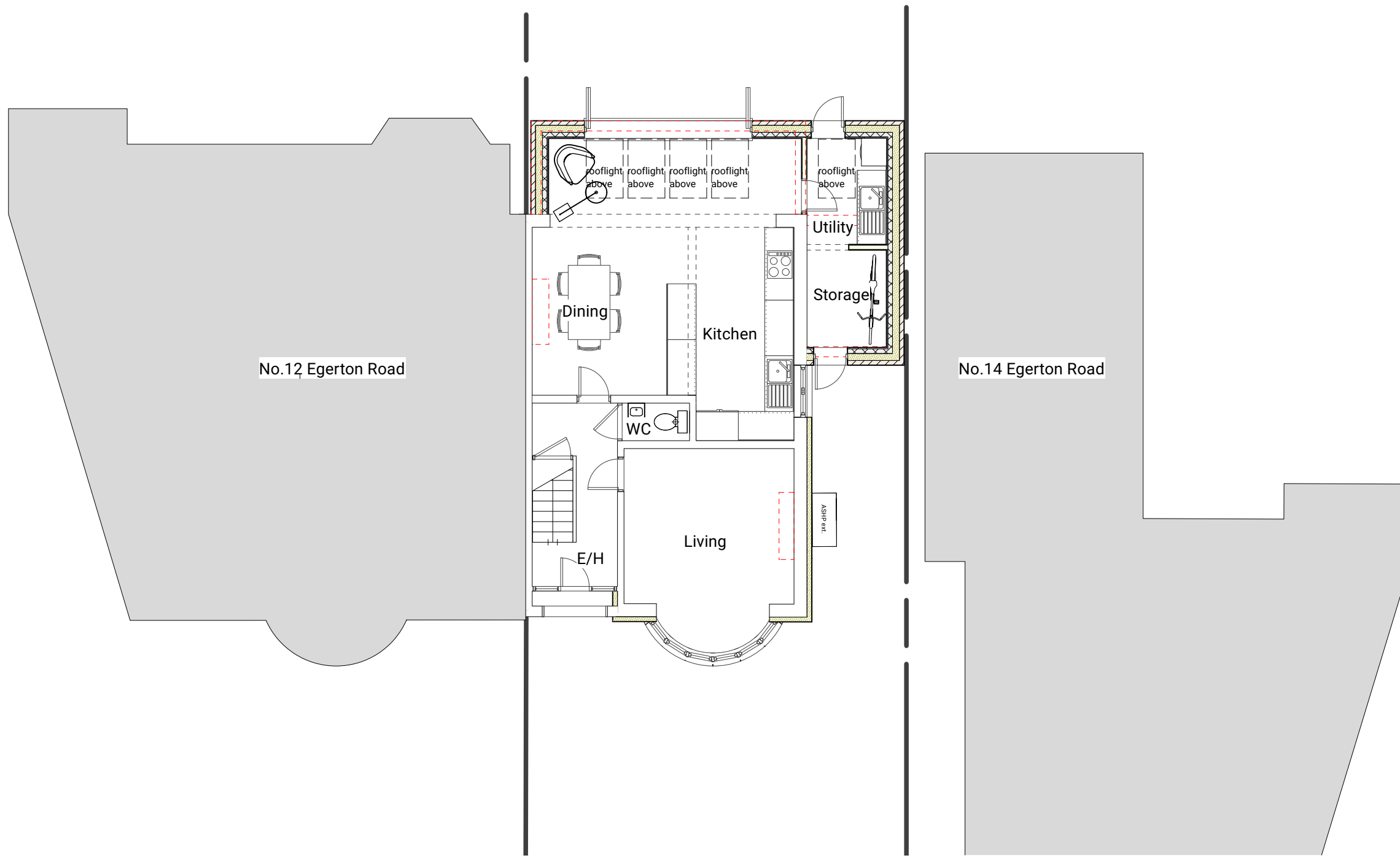
1 Ground Floor Plan Scale: 1:100
