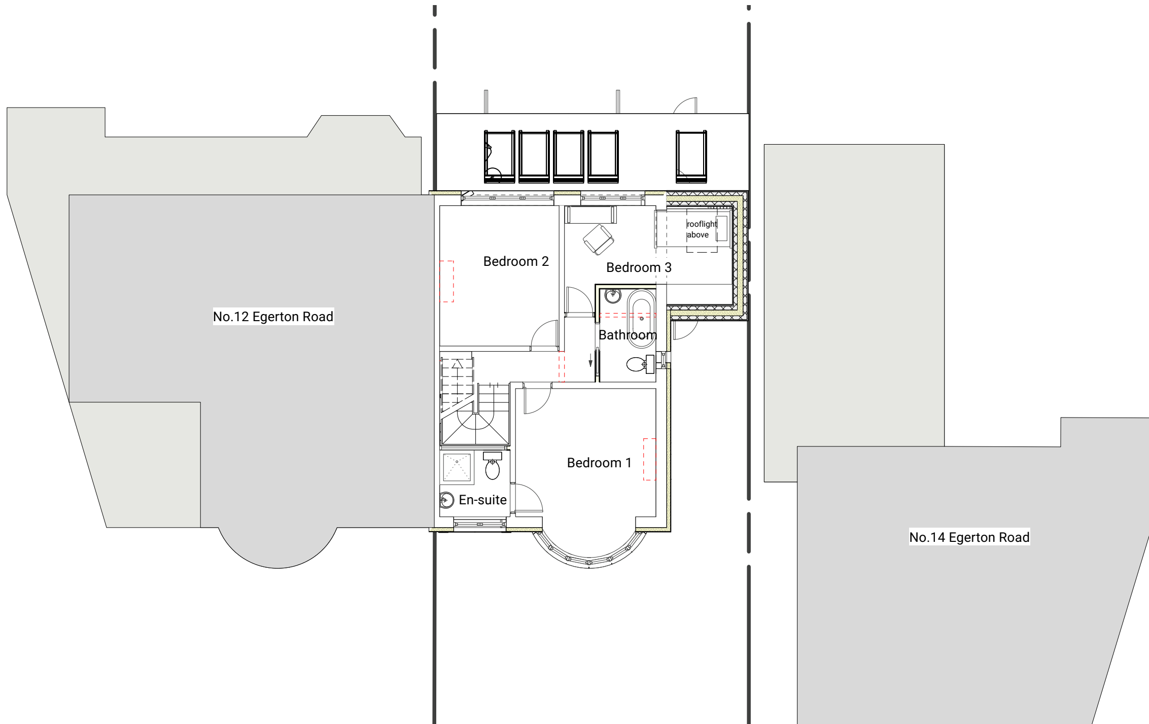
2 First Floor Plan Scale: 1:100
