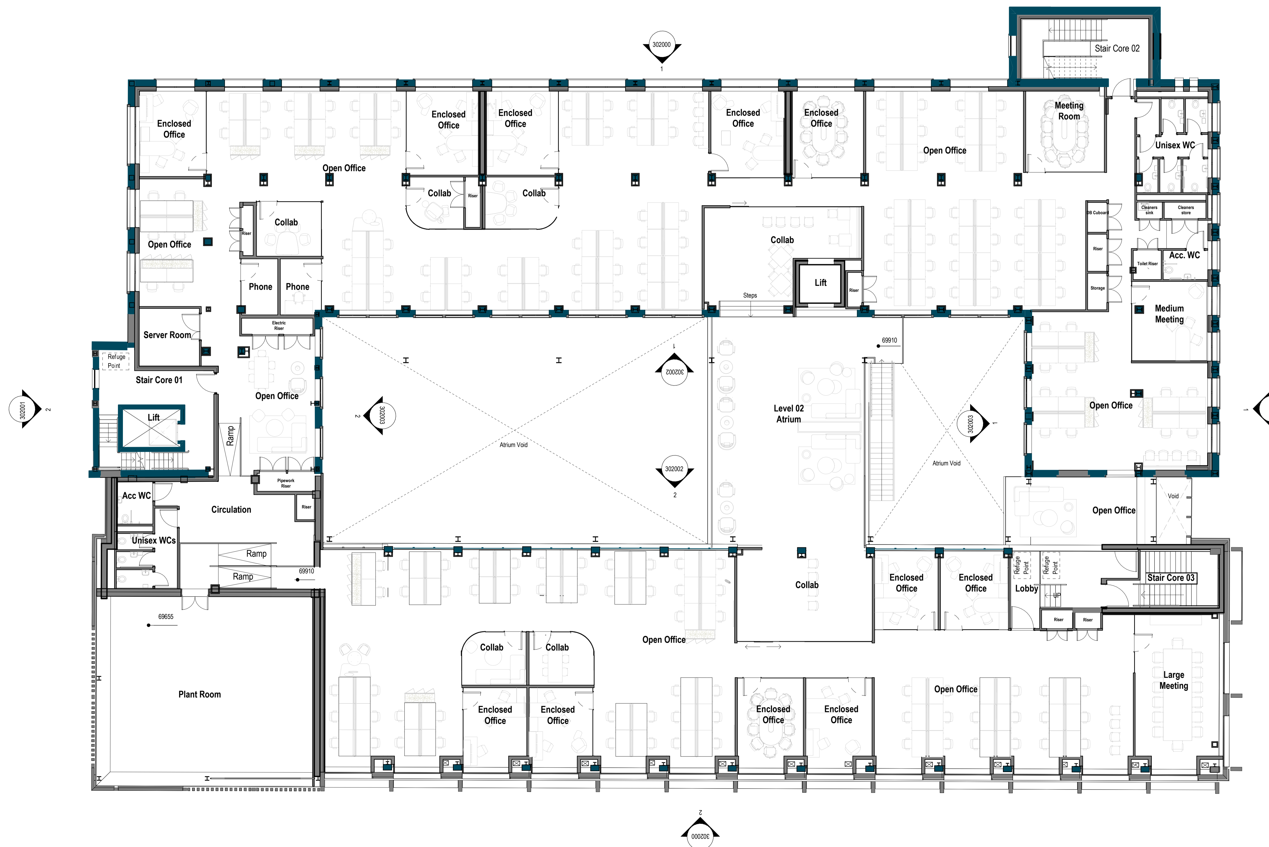
1 PROPOSED PLAN LAYOUT, LEVEL 02
