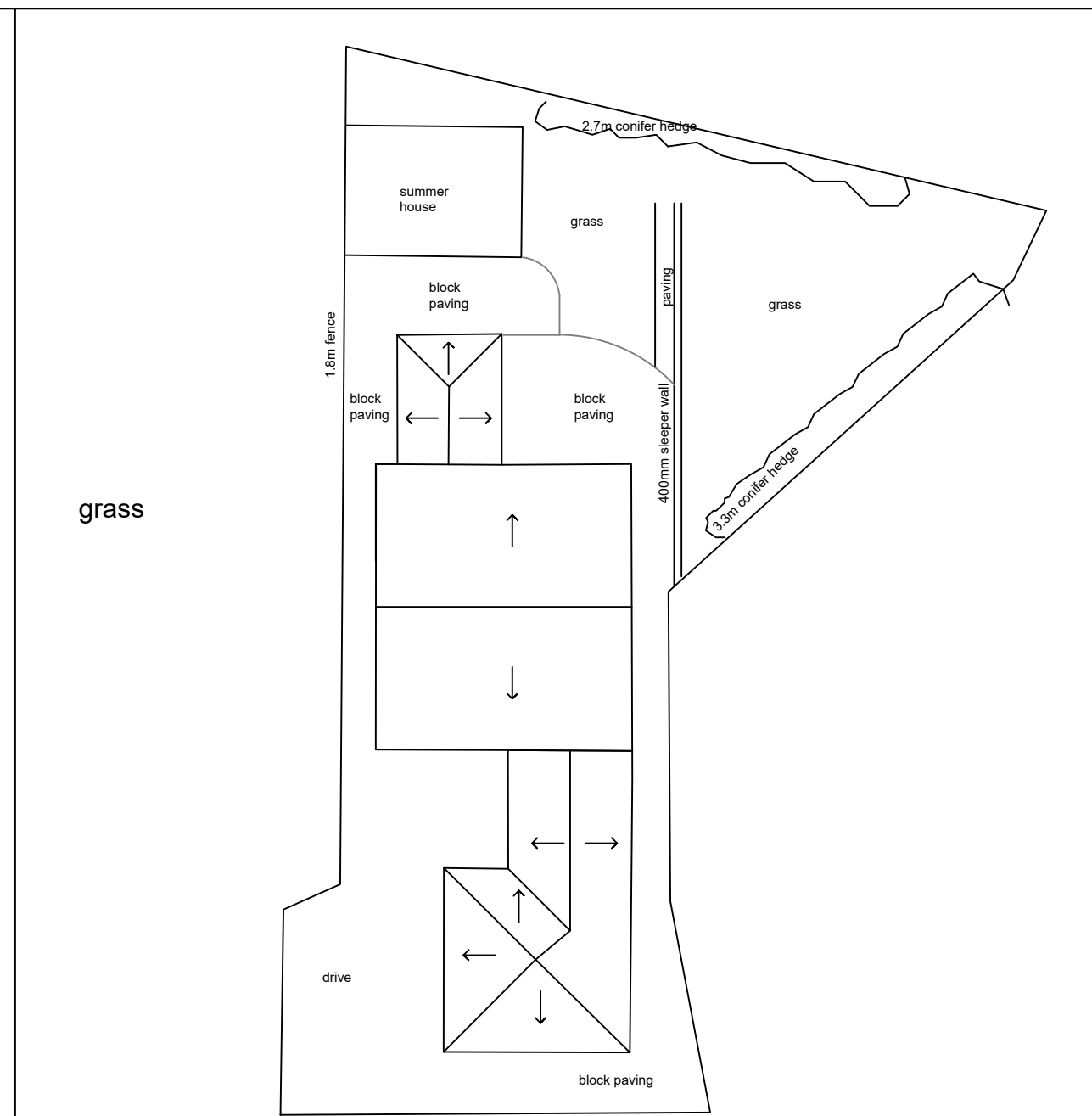
existing site and roof plan scale 1:200
