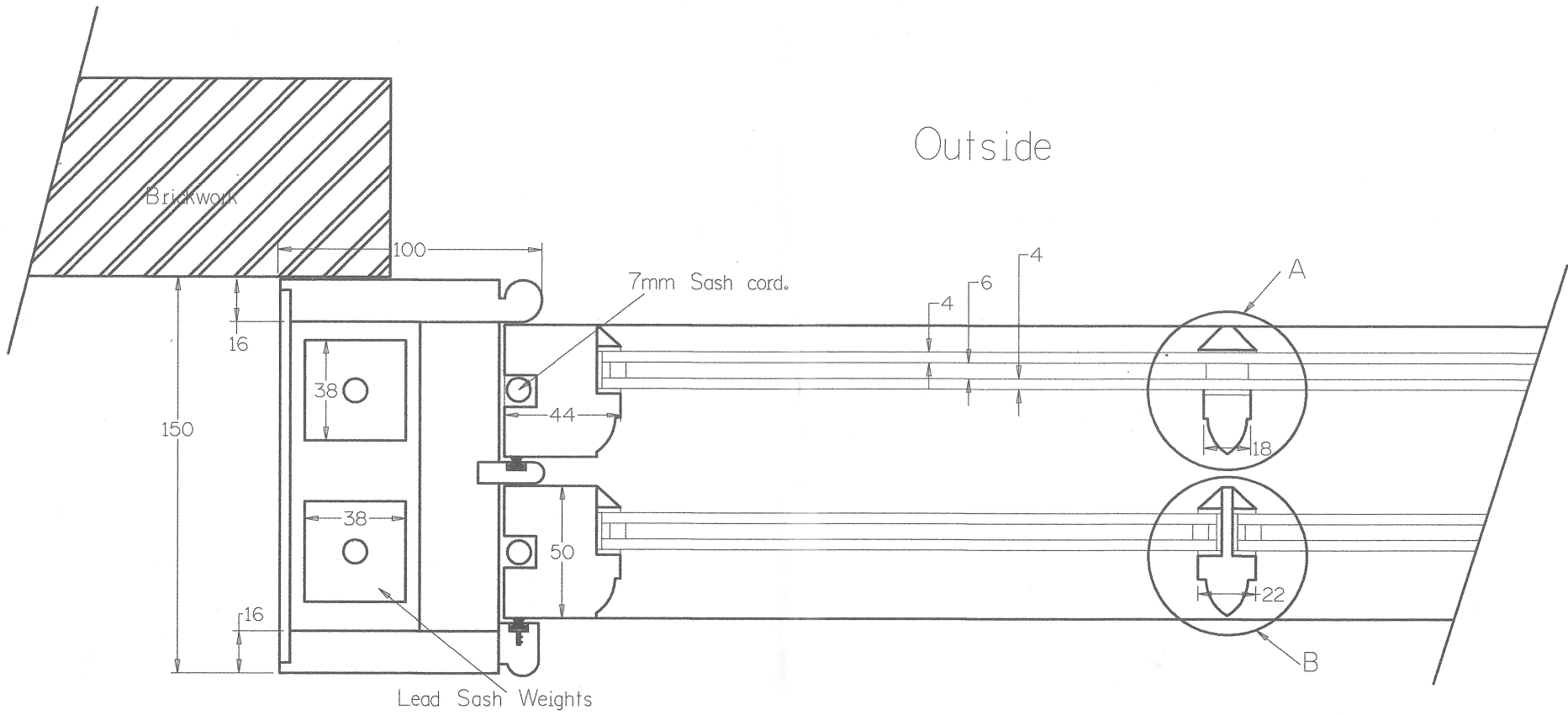
Section AA
