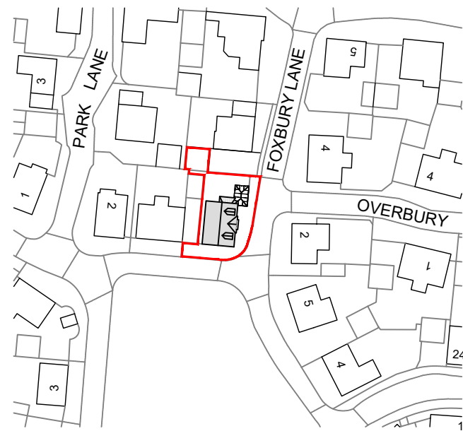
Location Plan 1:1250
