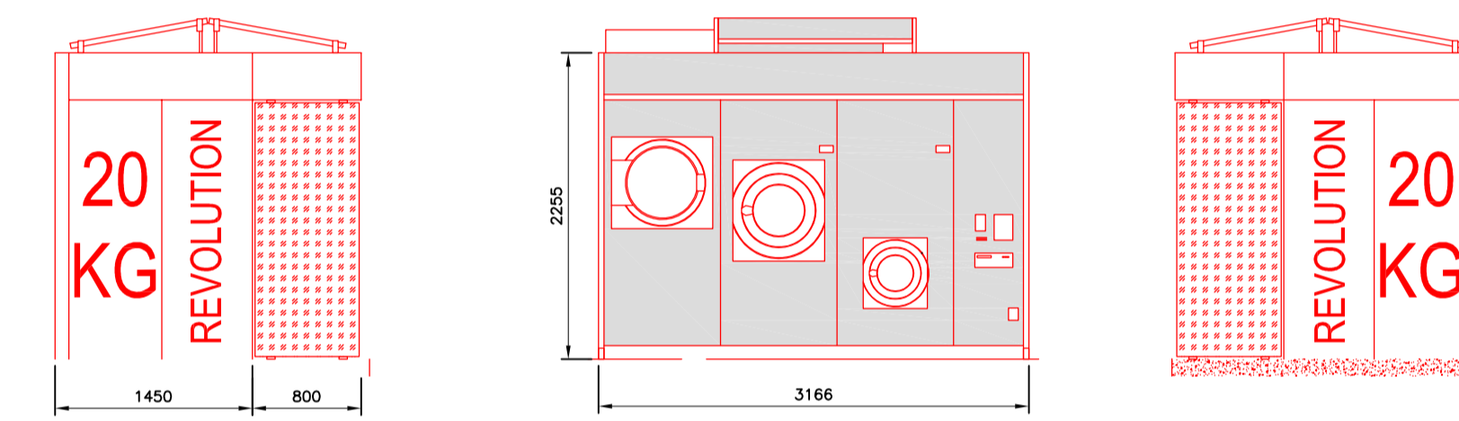
PROPOSED EXTERNAL LAUNDRETTE 1:50
