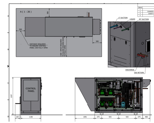
COMPRESSOR PACK
