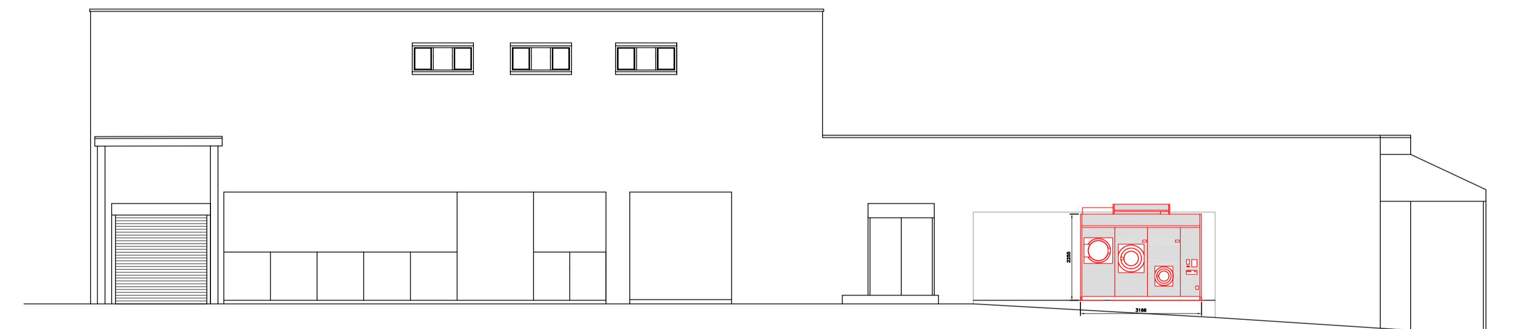
PROPOSED EXTERNAL LAUNDRETTE 1:50
