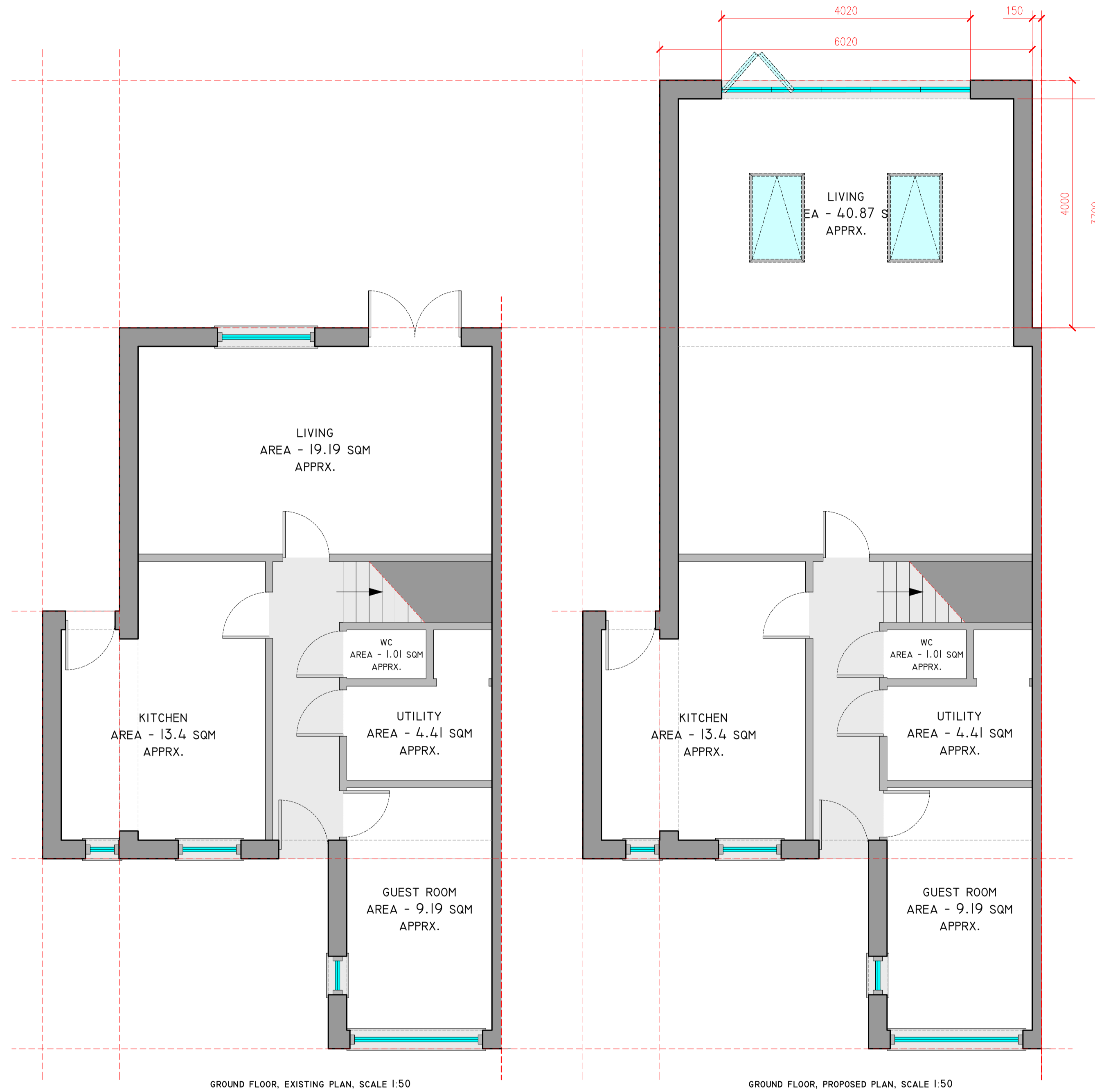
GROUND FLOOR, EXISTING PLAN, SCALE 1:50
